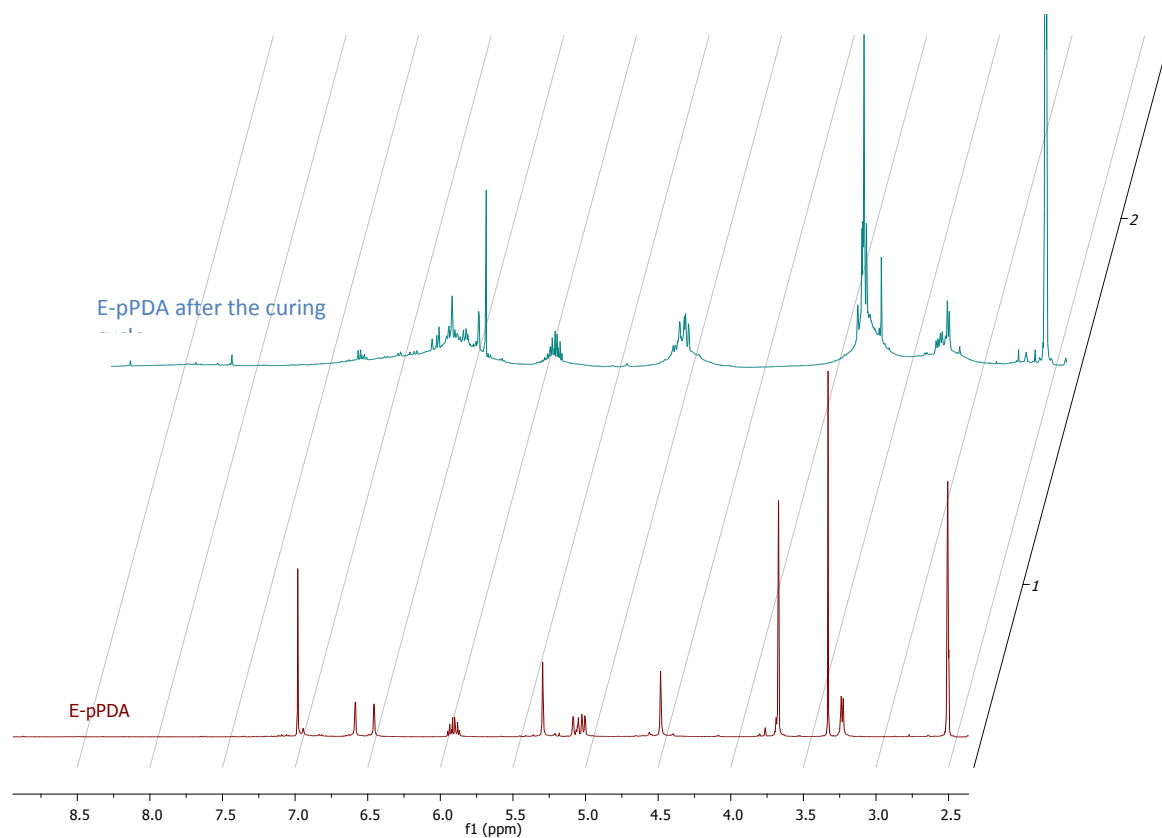
Fig. S1. 1 H NMR spectra of the E-pPDA monomer and E-pPDA after the curing cycle. DMSO-d 6
