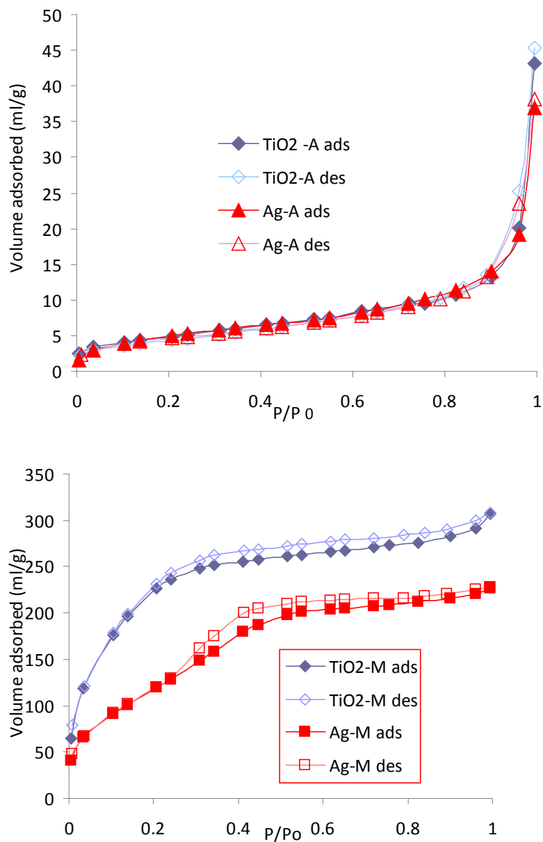
Figure SI-1. N 2 -adsorption-desorption isotherms of Ag-TiO 2 composites.
