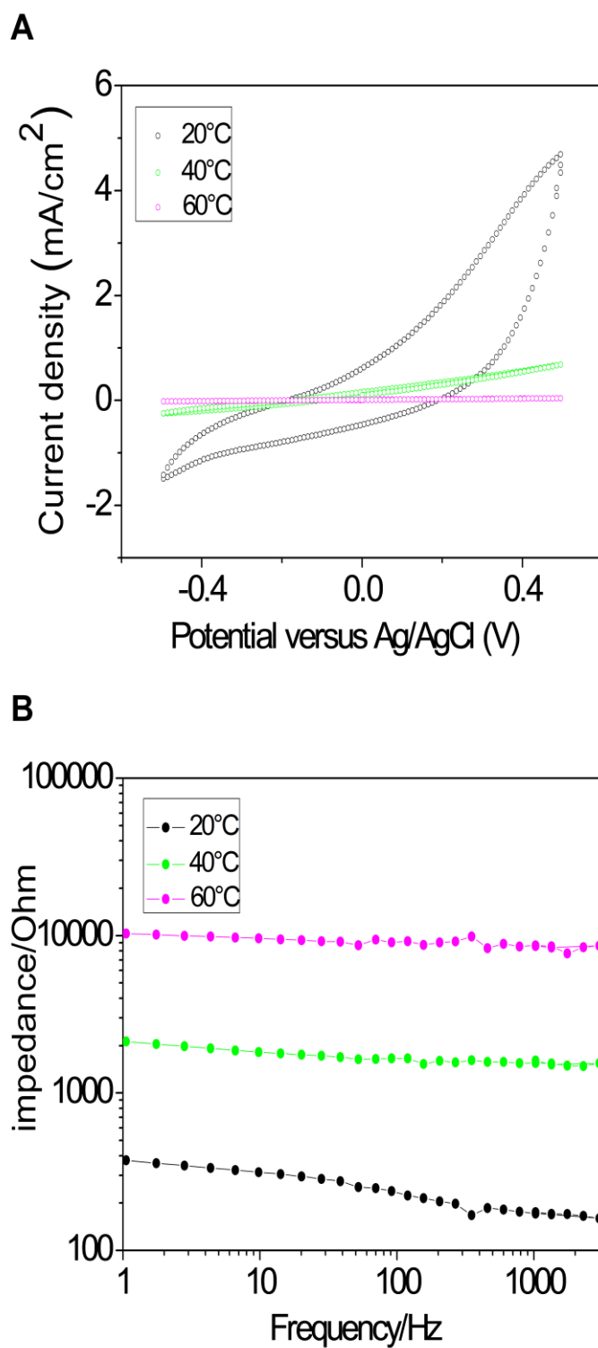
Figure S2. (A) Cyclic voltammety and (B) electrochemical impedance spectrum of PEDOT nanofiber mats obtained under different polymerization temperatures.
