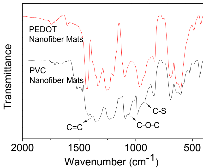
Figure S1. FTIR spectra of PVC nanofiber mats and PEDOT nanofiber mats.
