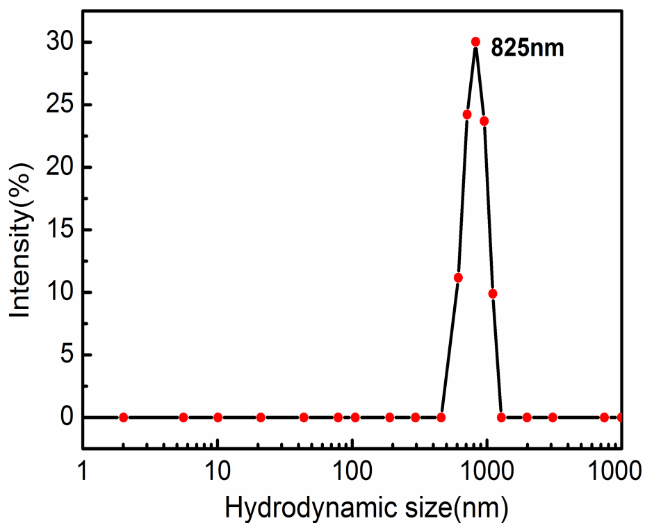
Fig.S1 The hydrodynamic size distribution of the GN-CNT-Fe 3 O 4
