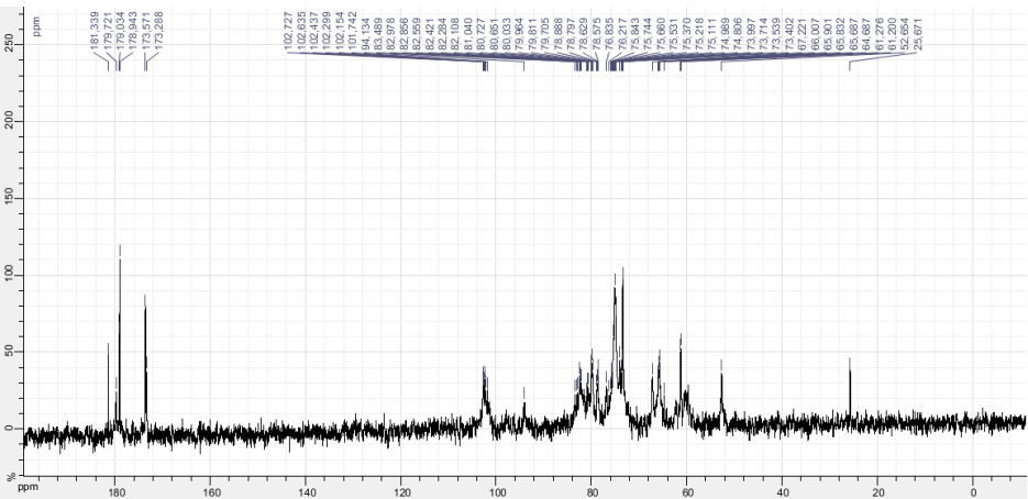
Figure 2S. 13 C NMR of CMC (D 2 O/HCl; 75 MHz)
