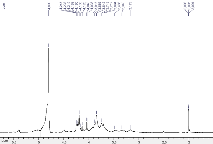
Figure 1S. 1 H NMR of CMC (D 2 O/HCl; 300 MHz)
