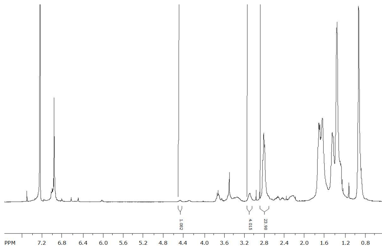
Figure 2: ^1\text{H} NMR spectrum of P3HT-biotin
