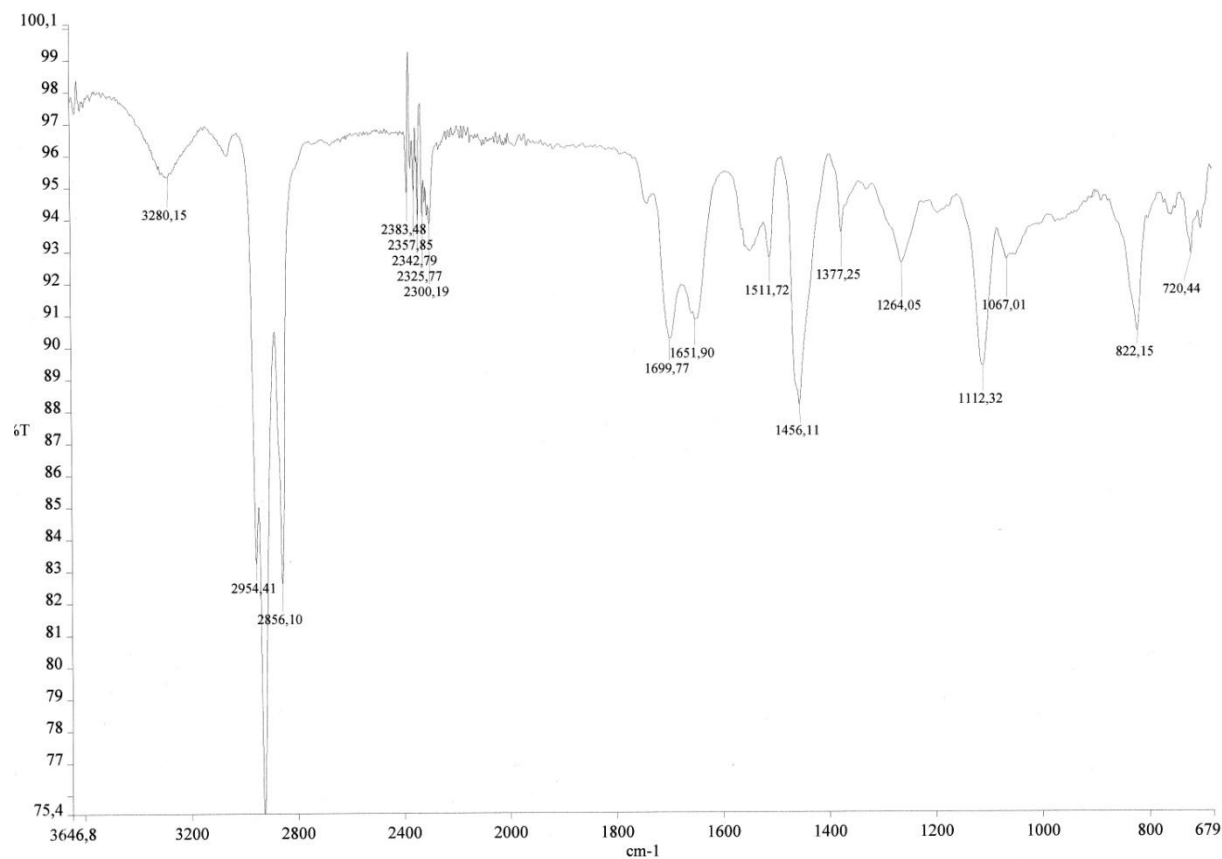
FT-IR spectrum of P3HT-biotin.
