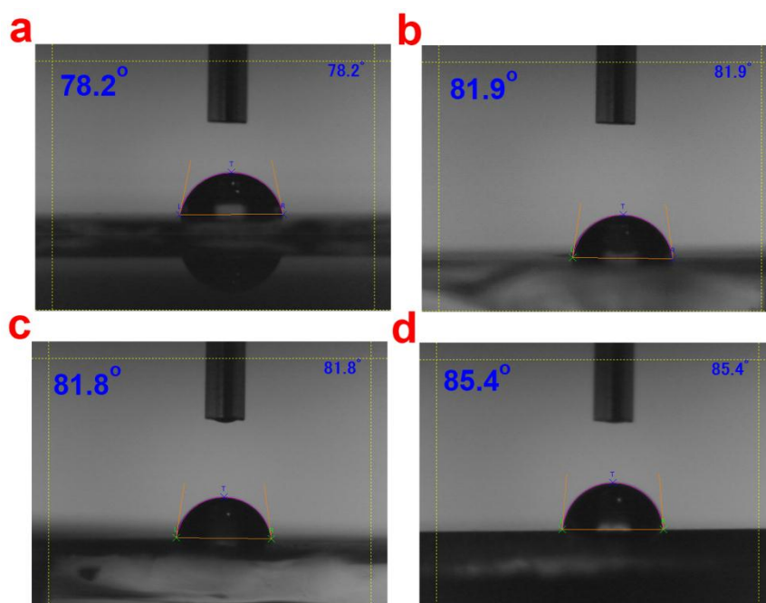
Figure S2. Water contact angles of the samples: (a) NGC-1; (b) MGR; (c) MGS; (d)
