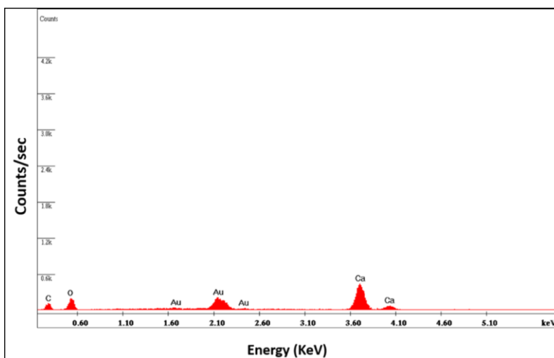
Figure S1: The EDS spectrum of hybrid CD-CaCO 3 microparticles.
