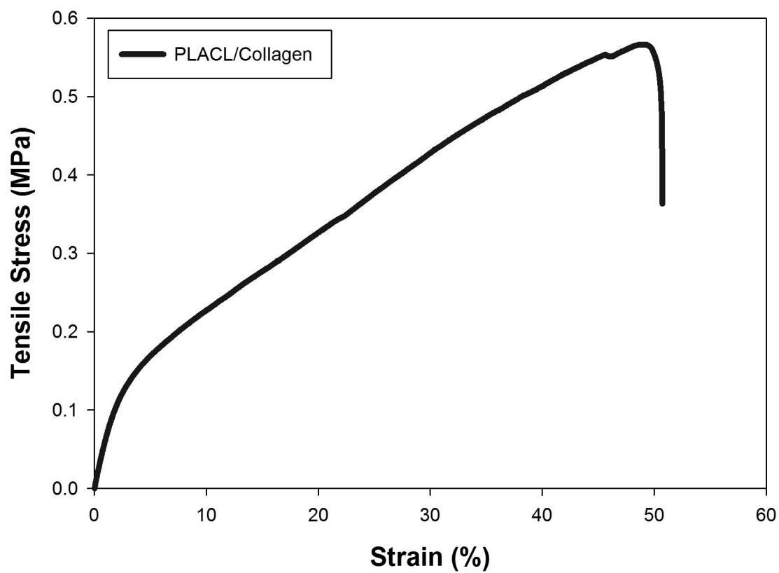
Figure S1. Stress-strain curve of PLACL/collagen nanofibrous scaffold.
