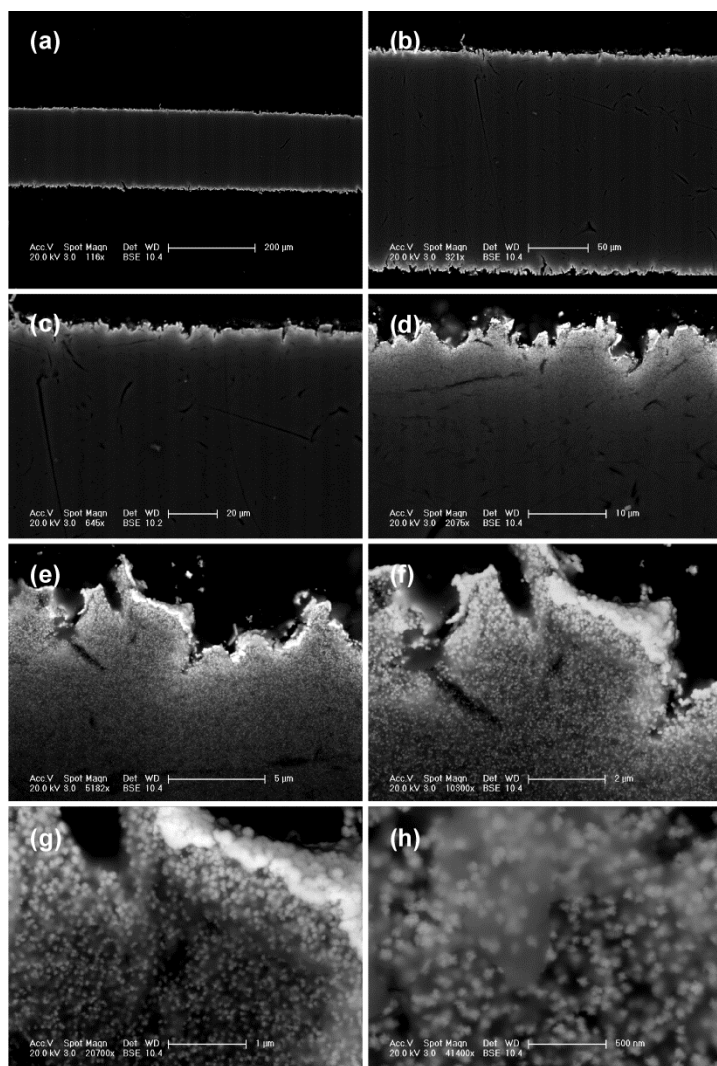
Figure S1. Back-Scattered Electron images of a cross-section of the IPMC sample Pt 1 Com taken at increasing magnifications showing the porous electrode structure and the individual Pt clusters.
