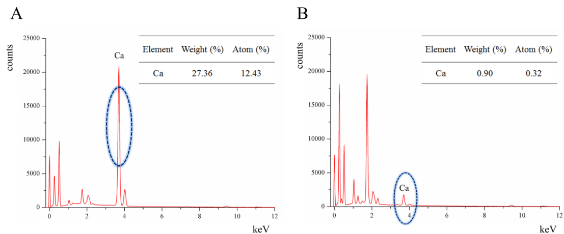
Fig. S1. The energy-dispersive X-ray analysis of (A) \text{CaCO}_3 (BSA) particles and (B) BSA-gel-capsules(MPs). There was little calcium in BSA-gel-capsules(MPs), indicating that \text{CaCO}_3 was almost completely removed after treatment with EDTA.
