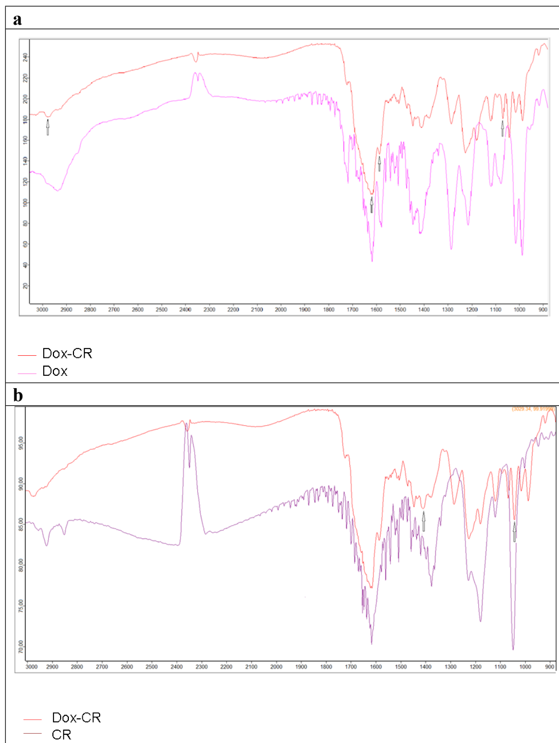
Fig. 8 a. FTIR spectra of Doxorubicin like free molecule (pink line) and FTIR spectra of Doxorubicin with Congo Red (red line). b. FTIR spectra of Congo Red like free molecule (violet line) and FTIR spectra of Doxorubicin with Congo Red (red line).
