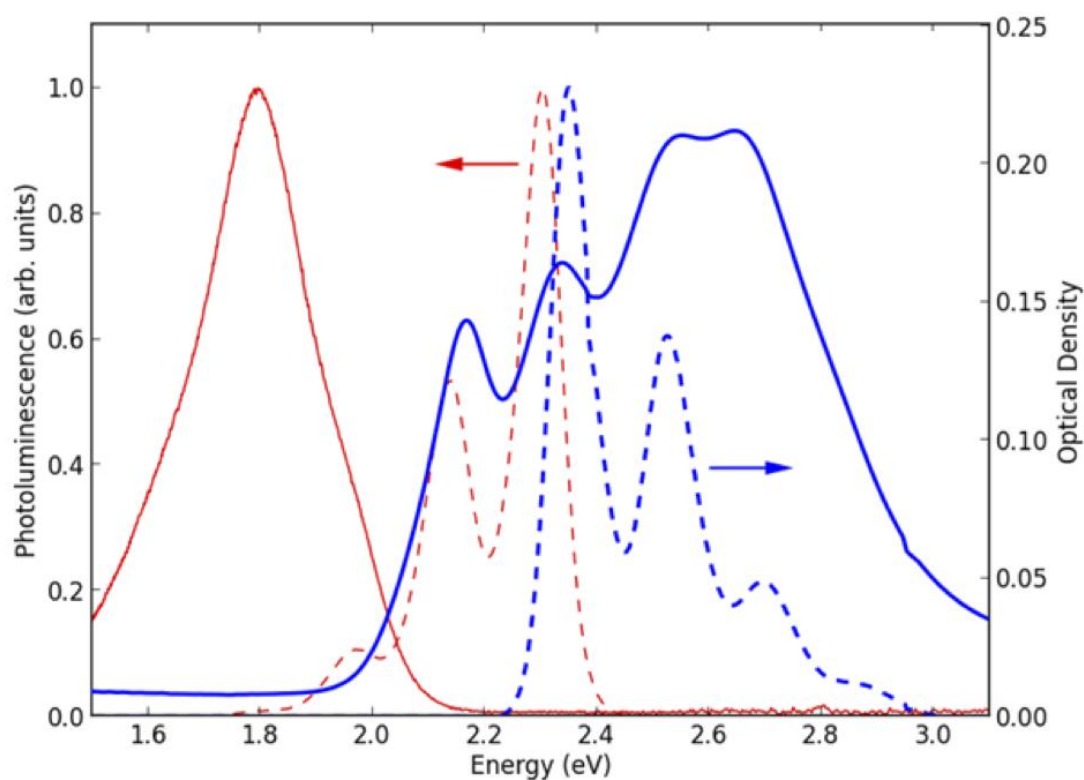
Figure S1. Absorption (blue lines) and photoluminescence (red lines) spectra of P13 in solution (dashed lines) and in thin-film on quartz (solid lines). The differences between the thin-film and the solution spectra indicate the high degree of intermolecular interaction in the condensed phase.
