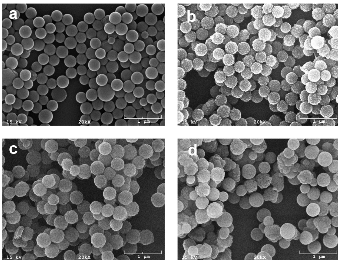
Fig. S1 Low magnification SEM images of hollow silica spheres obtained at various amounts of TEOS. (a) 0.5 \mu l. (b) 1 \mu l. (c) 2 \mu l. (d) 4 \mu l
