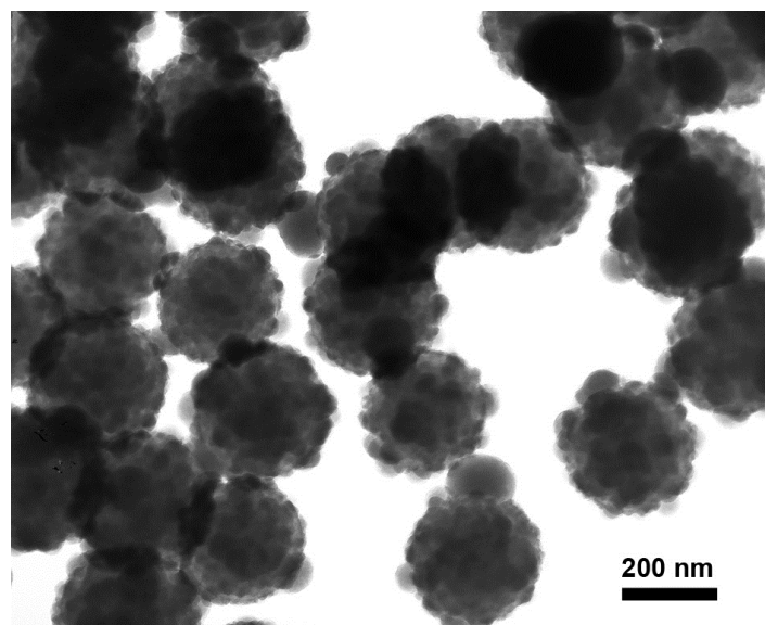
Fig. S5 TEM micrographs of the silica spheres on amino-PS templates. To produce them, 10^{-2} mmol APTES was mixed first with 500 \mu\text{l} of PS particles first and then with 1 \mu\text{l} of TEOS. A rougher surface of silica spheres with some free silica particles attached was observed.
