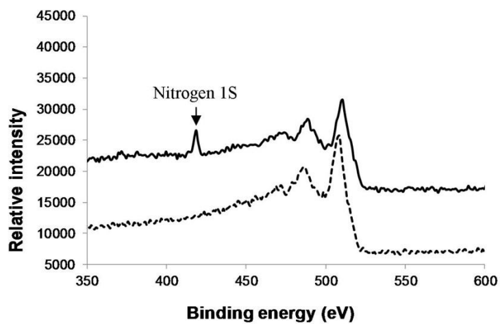
Fig. S1 XPS spectra of AGE-coated (dotted lines) and AGE-Pmpi-coated (solid lines) silicon wafers
