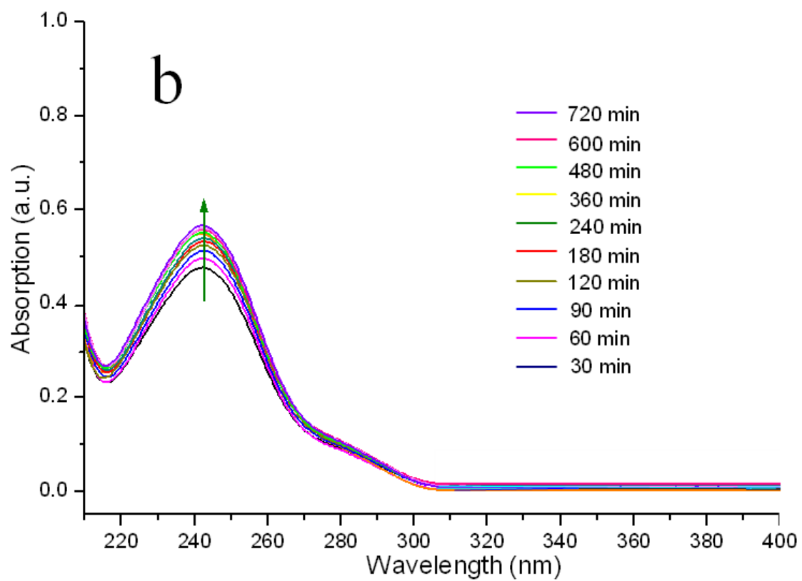
Figure S1. UV-vis spectra changing with time: (a) Ac loading and (b) release process of Ac in S3.
