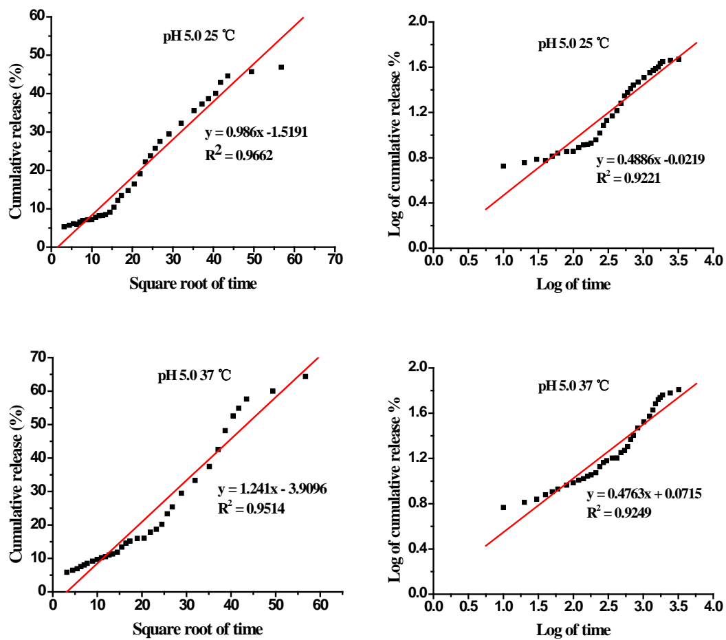
Figure S1. The curve of Higuchi and Korsmeyer-Peppas equation models mechanism of drug release.
