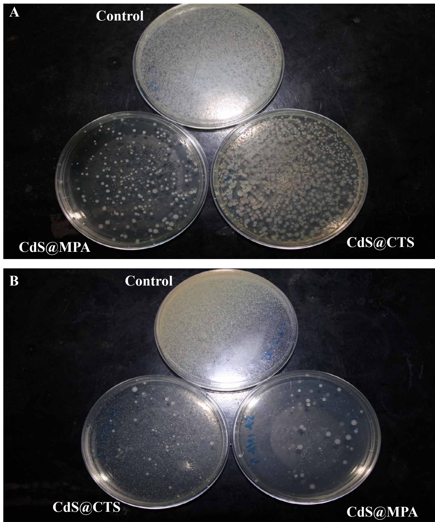
Figure S2: Plate counting of P. aeruginosa (A) and S. aureus (B)
