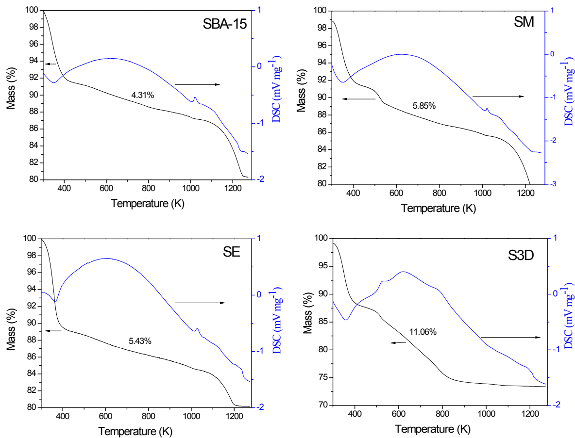
Figure S5. TG-DSC measurements of samples SBA-15 containing heparin.
