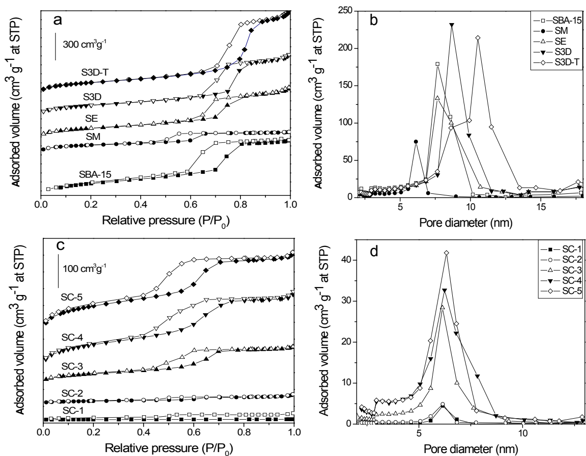
Figure S4. The N 2 adsorption–desorption isotherms (a, c) and pore size distribution (b, d) of SBA-15 sample with different morphologies (a, b), carbonized SM (SC-n) samples (c, d).
