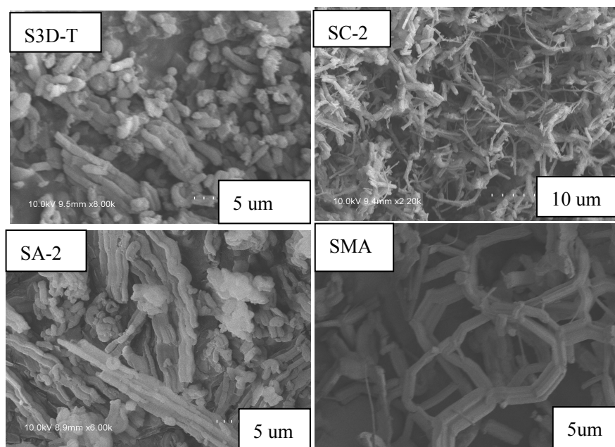
Figure S1. The SEM images of SBA-15 analogues samples.
