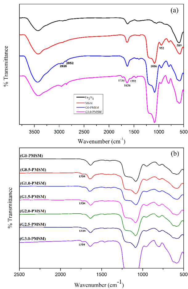
Fig. S1 FT-IR spectra of the preparation of dendrimer-modified magnetic microspheres (a) and different generations of PAMAM on PMSM (b).
