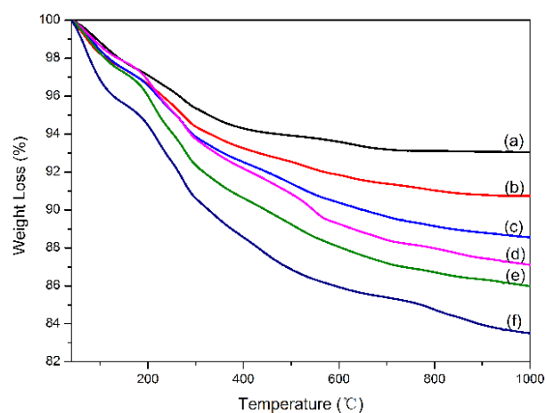
Fig. S2 TGA curves of MSM (a), G0-PMSM (b), G1.0-PMSM (c), G2.0-PMSM (d), G3.0-PMSM (e) and HSA-PMSM (f).
