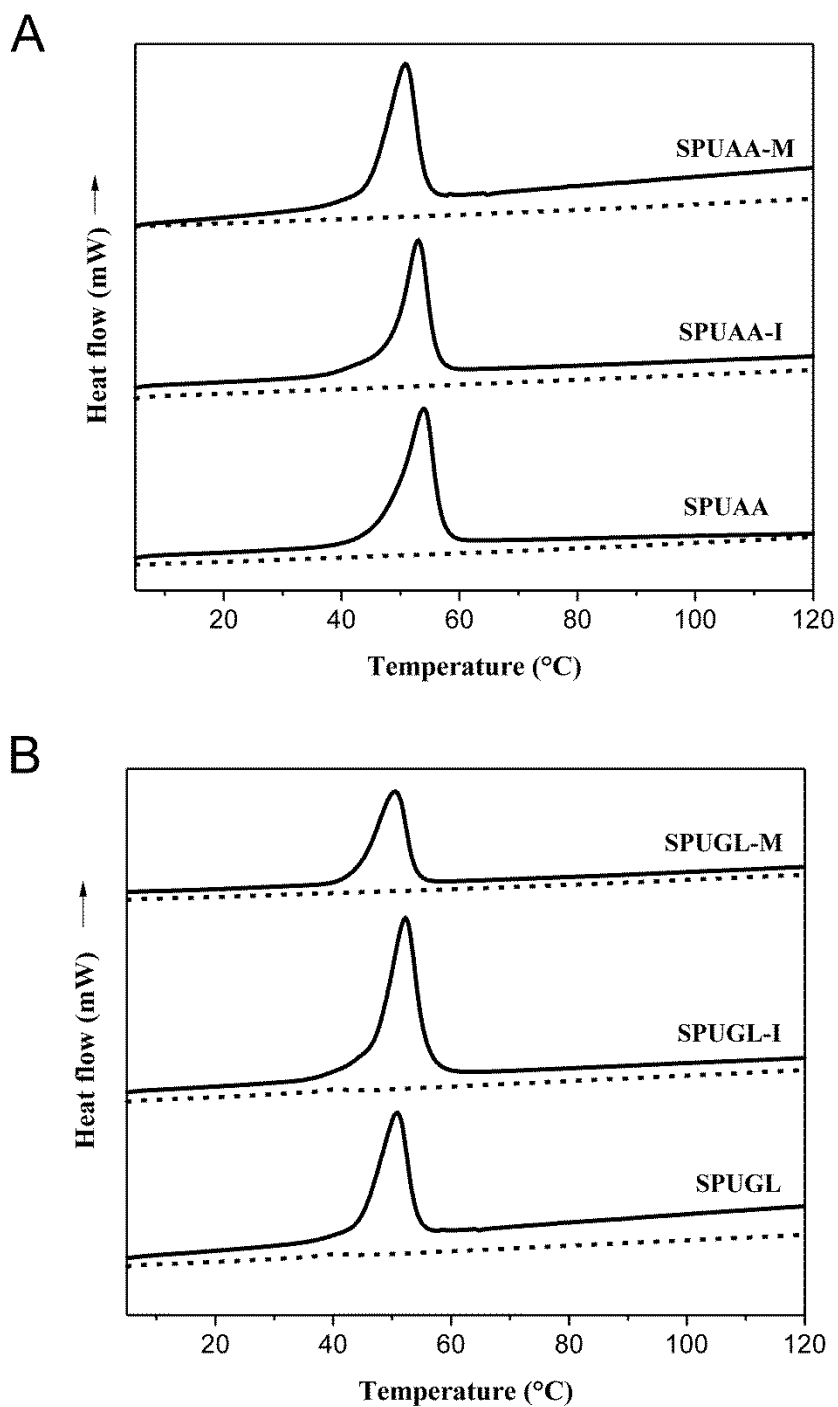
S-1. DSC Termograms. First (—) and second(----) heating
