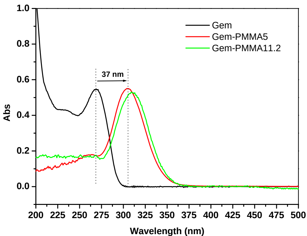
Figure 1. The UV-Vis curves of free gemcitabine and Gem-PMMA conjugates.
