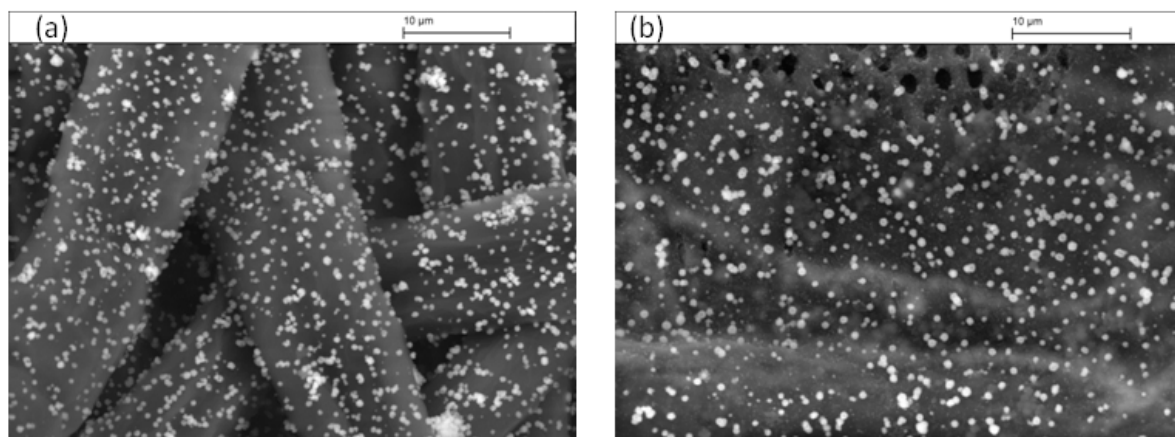
Fig. 1 SEM images of the ZnO/CMS loaded papers (a) before antibacterial test and (b) after antibacterial test and ethanol washing.
