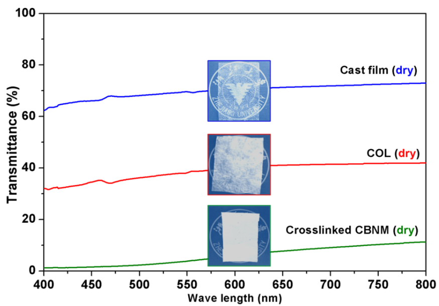
Fig. S2. Light transmittance of cast film, pure COL membrane and GA-crosslinked CBNM in dry state.
