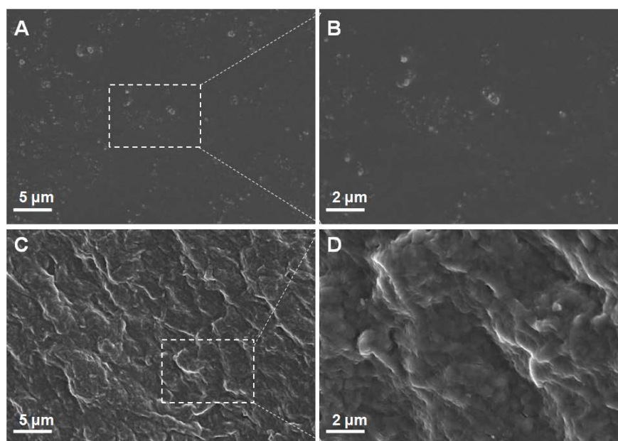
Fig. S1. SEM images of the film-cast COL-HA-PEO films (A, B) and their CS-modified membranes (C, D).
