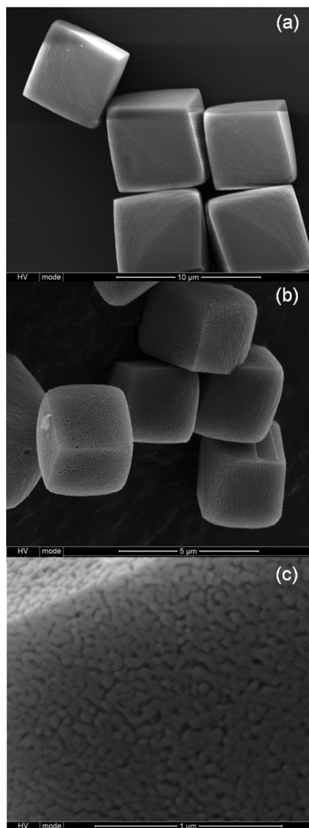
Figure S1. SEM images of 4 μm cubic manganese carbonate particles before (a) and after (b, c) heating at 700°C for 3 hours in air.
