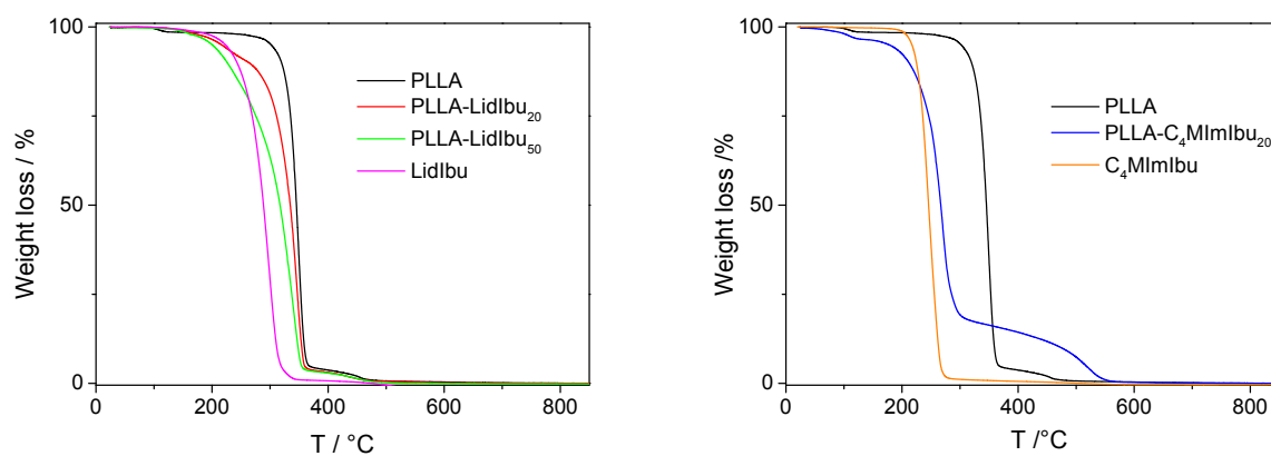
Figure S2. Left : TGA curves of (-) PLLA, (-) LidIbu , (-) PLLALidIbu_{20} and (-) PLLALidIbu_{50} before release experiments. Right : TGA curves of (-) PLLA, (-) C_4MImIbu and (-) PLLAC_4MImIbu_{20} before release experiments.
