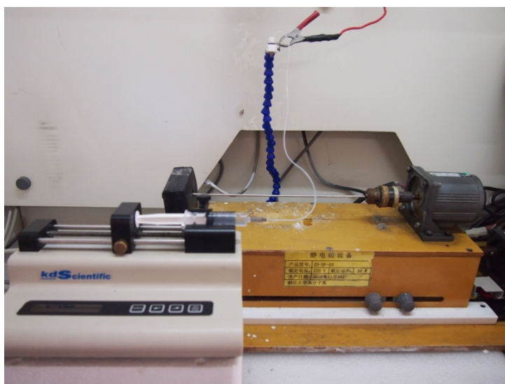
Figure S1. The picture of electrospinning instruments used in this study.
