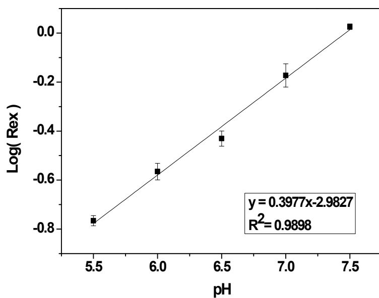
Figure S1. Calibration curve of Rex Value with intracellular pH, which obtained in different pH buffer.
