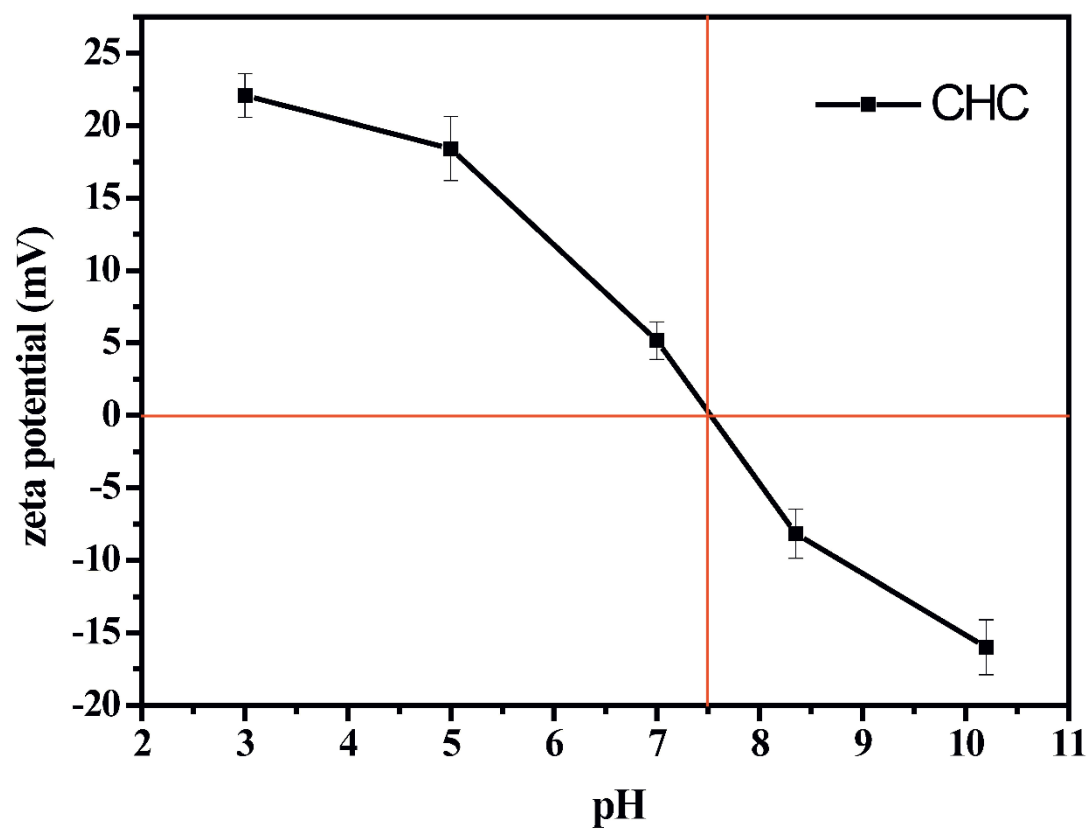
Figure S2. The zeta potential curve of CHC core nanoparticle, where an IEP is determined at ~pH 7.5.
