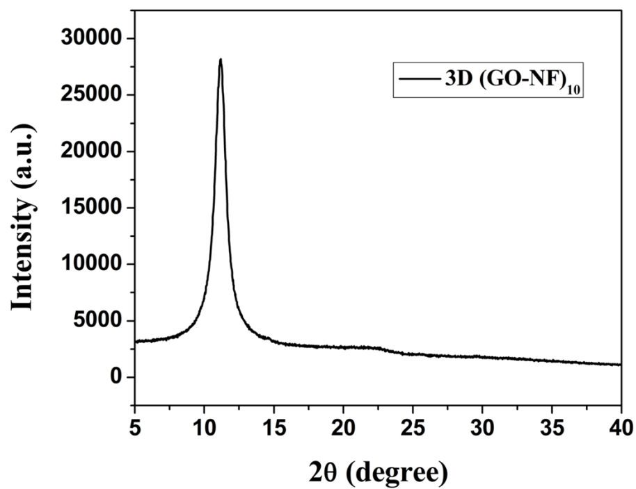
Fig. S2 XRD pattern of the fabricated 3D (GO-NF) 10 scaffold.
