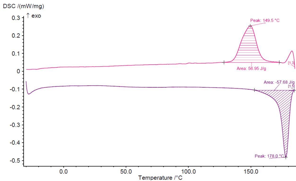
Figure 6: DSC curve of espun PLLA/PMeDX (100/0)
