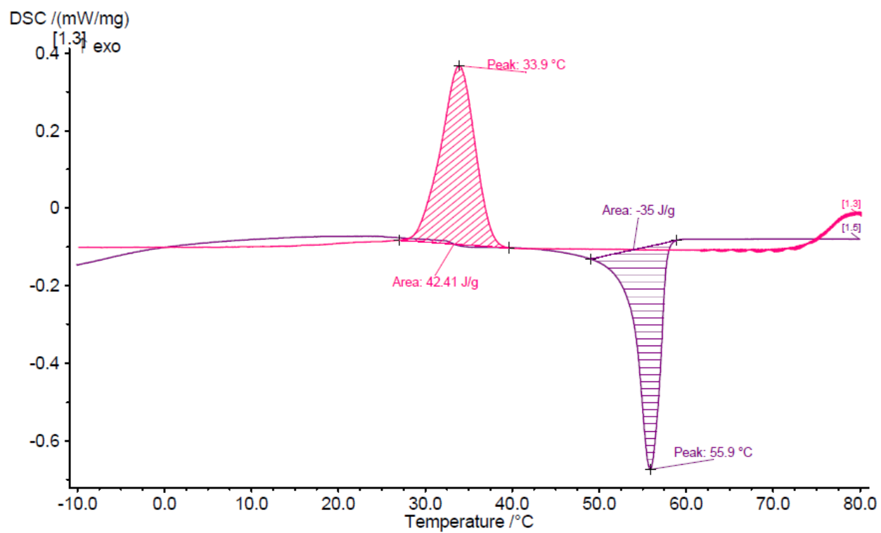
Figure 5: DSC curve of espun PCL/PMeDX (85/15)
