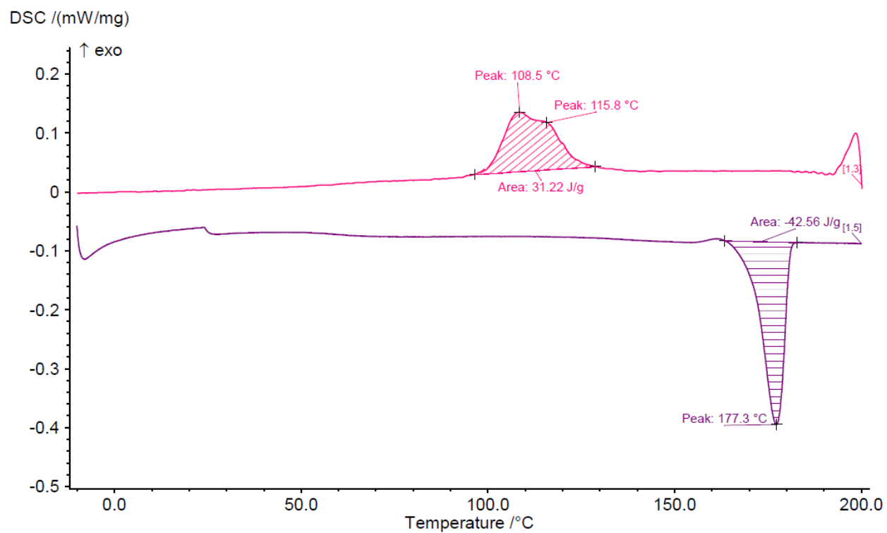
Figure 10: DSC curve of espun PLLA/PMedX (85/15)
