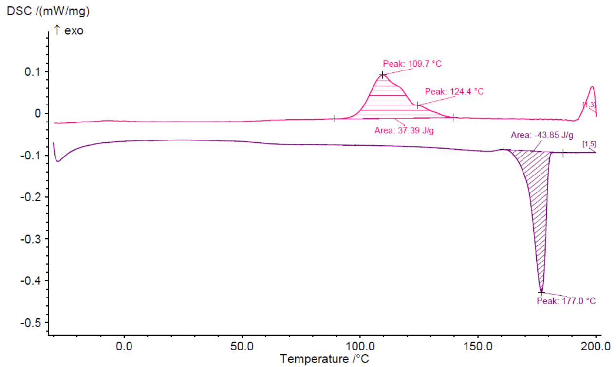
Figure 9: DSC curve of espun PLLA/PMeDX (90/10)
