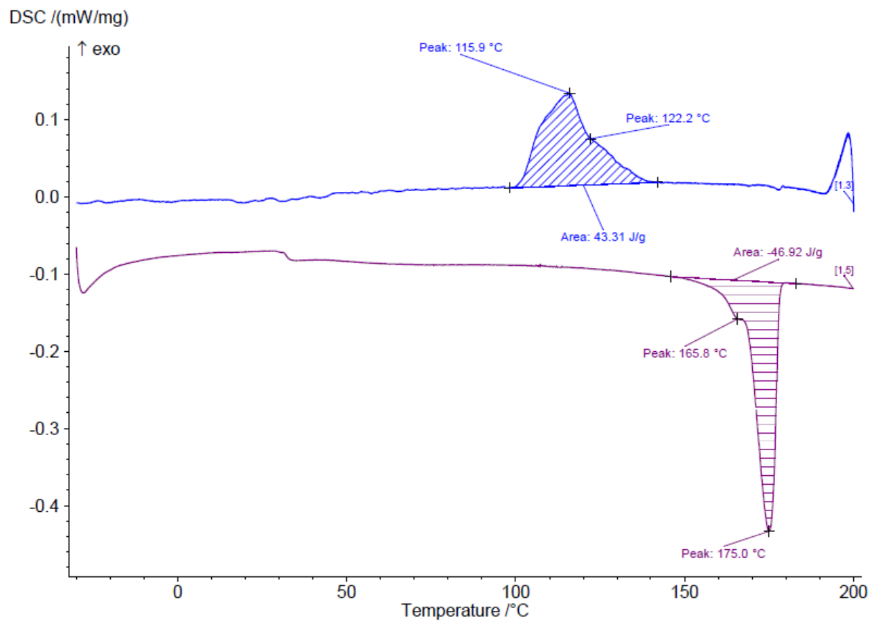
Figure 7: DSC curve of espun PLLA/PMedX (98/2)
