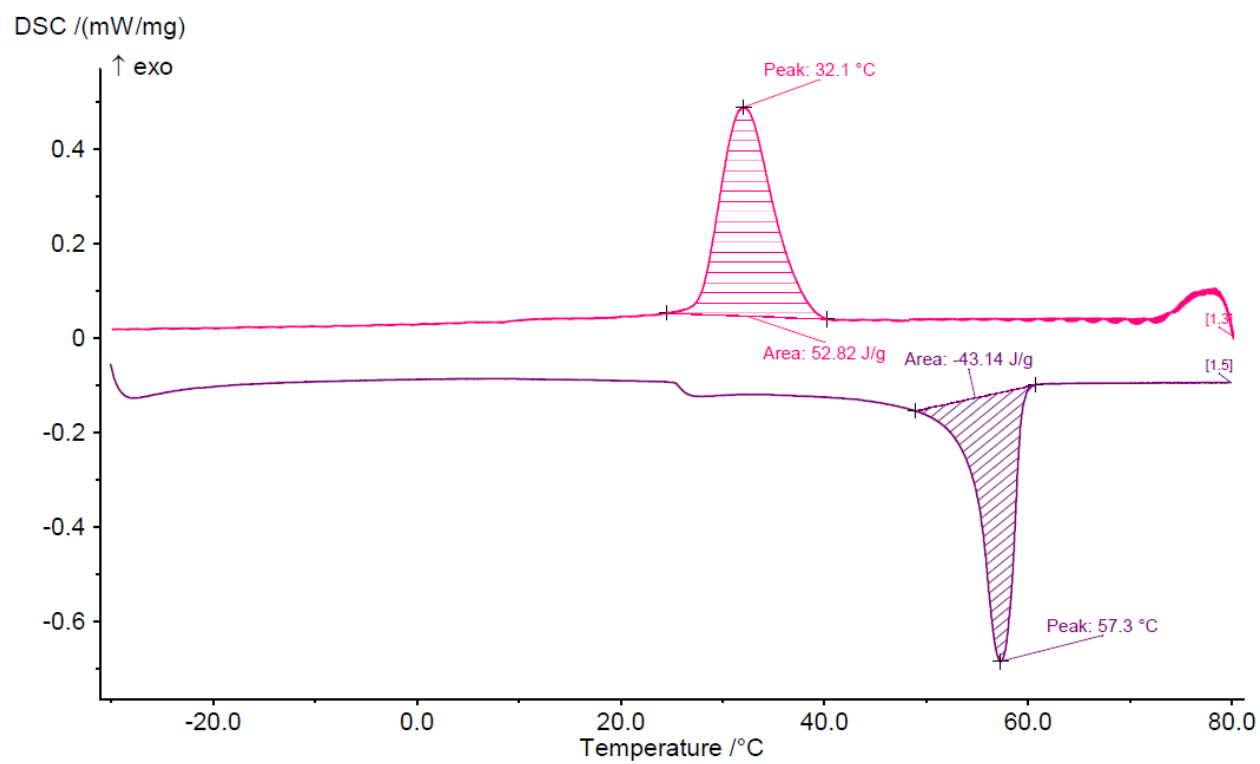
Figure 2: DSC curve of espun PCL/PMedX (98/2)
