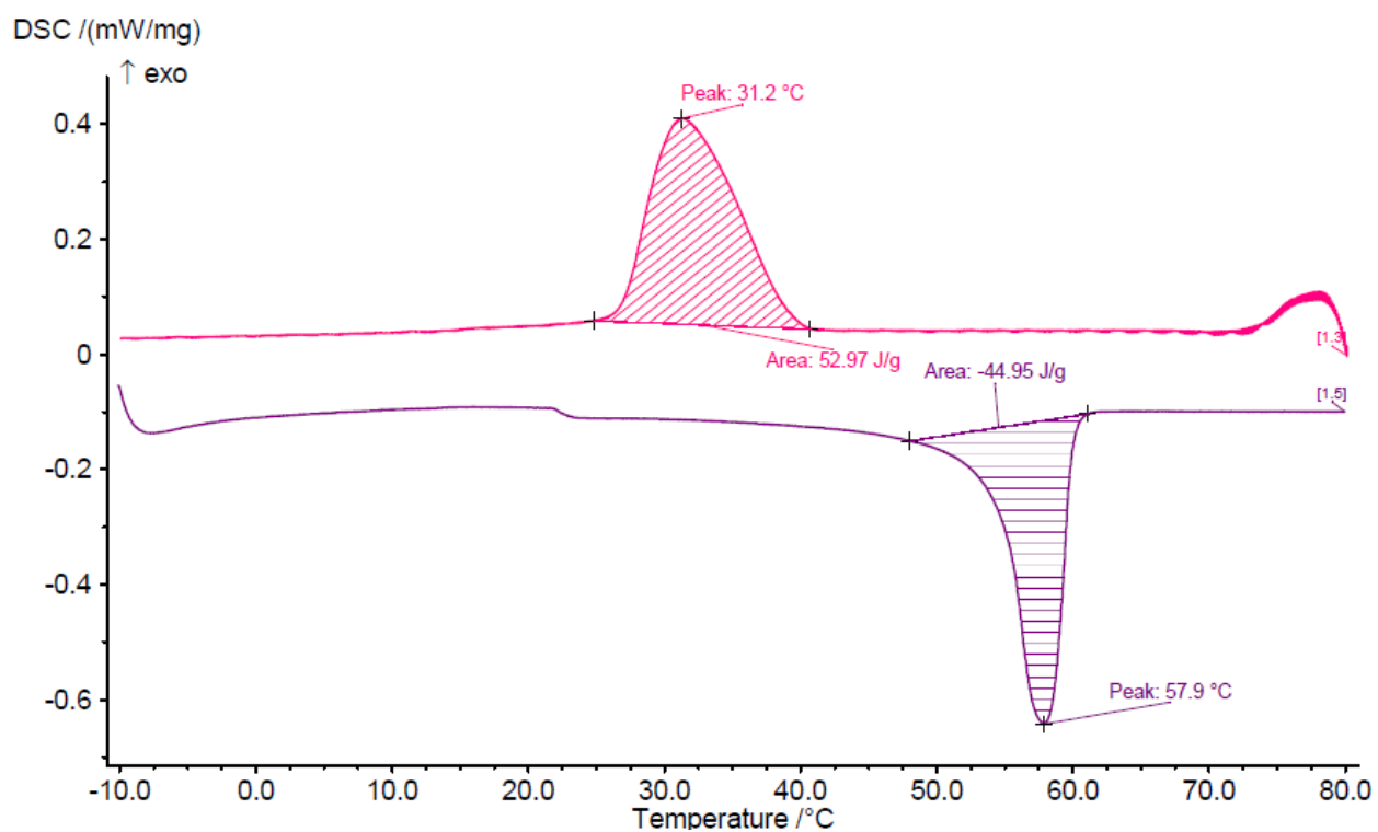
Figure 1: DSC curve of espun PCL/PMedX (100/0)
