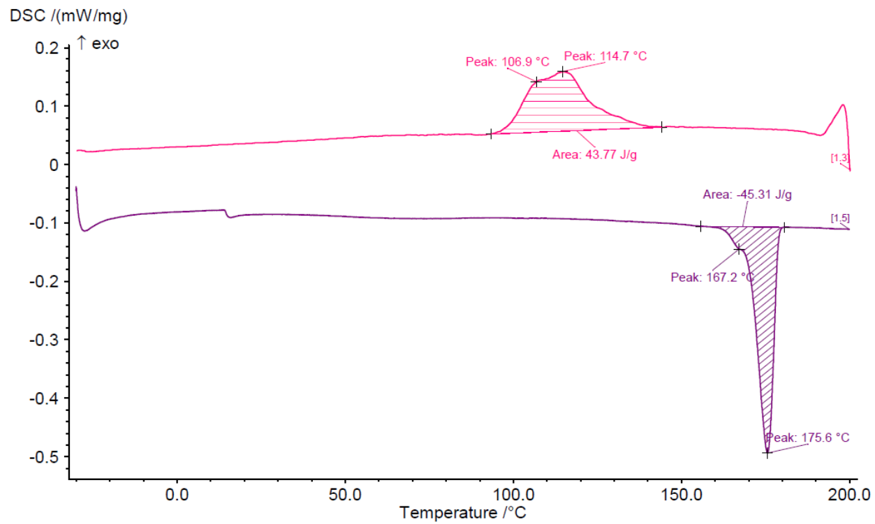
Figure 8: DSC curve of espun PLLA/PMedX (93/7)
