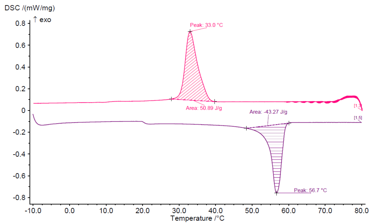
Figure 3: DSC curve of espun PCL/PMeDX (93/7)
