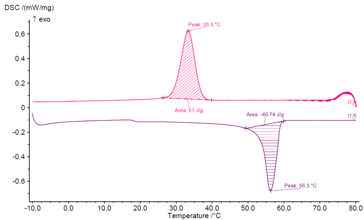
Figure 4: DSC curve of espun PCL/PMeDX (90/10)
