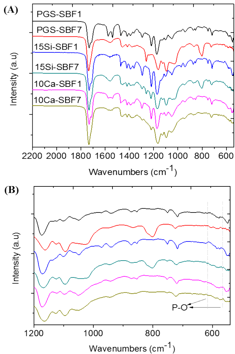
Figure S1. FTIR spectra of samples after soaking in SBF for 1 and 7days.
