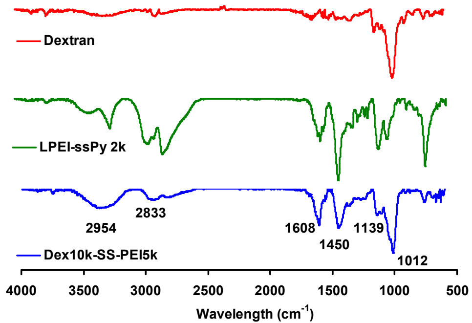
Figure S2. FT-IR spectrum of dextran, 2kDa PEI disulfide pyridine and Dex10k-SS-PEI5k.
