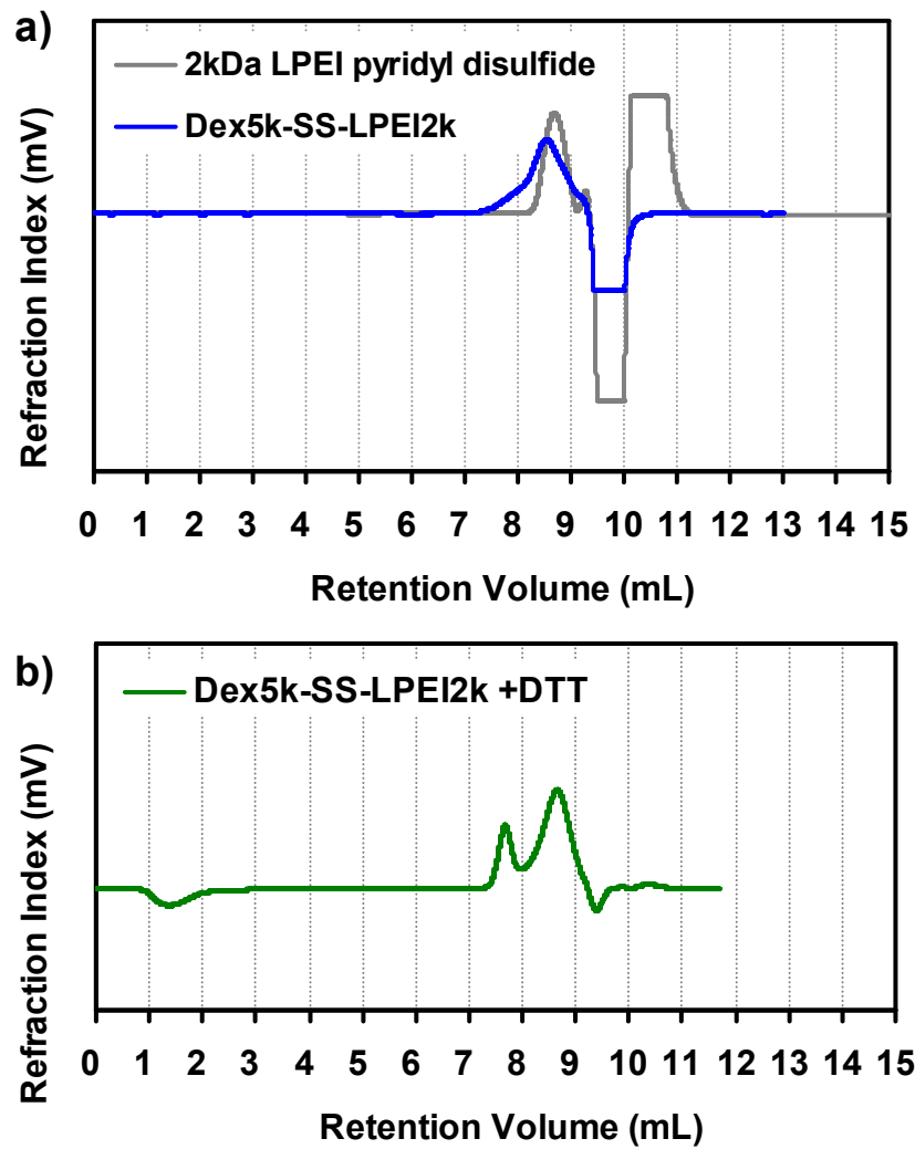
Figure S1. a) GPC profile of Dex5k-SS-LPEI2k and 2kDa LPEI disulfide pyridine; b) GPC profile of Dex5k-SS-LPEI2k in the presence of 2.5 mM dithiothreitol (DTT)
