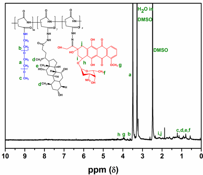
Figure S2. 1 H-NMR spectra of MPEG/CA10/DOX-g-PASPAM.
