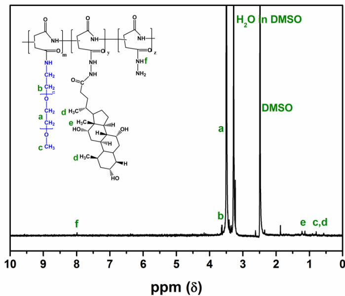
Figure S1. 1 H-NMR spectra of MPEG/CA10/Hyd-g-PASPAM .
