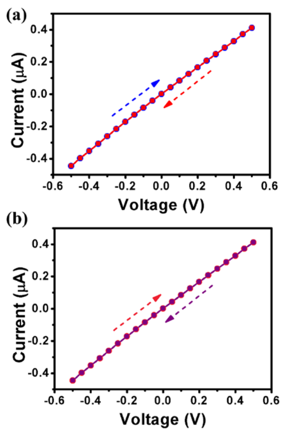
Figure S1. Reciprocating scan on a single ZnS:Cu NR with both ohmic contacts at two ends. The voltage sweeping speed are (a) +0.5 \text{ V s}^{-1} and (b) +0.05 \text{ V s}^{-1} , respectively.
