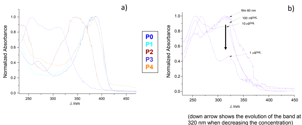
Figure S1. left: absorption spectra of P0–P4 (10 μg/mL in CH 2 Cl 2 ); right: absorption spectrum of P3 at different concentrations.
