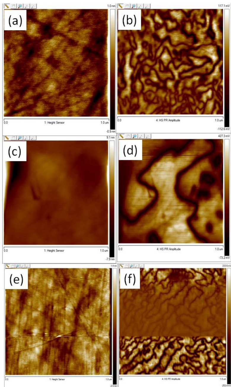
Figure S-1 (a)-(b), (c)-(d) and (e)- (f) Height and amplitude PFM images corresponding to the phase image showing domain structure in figure 6(e), inset of figure 6(e), and figure 6(f), respectively.
