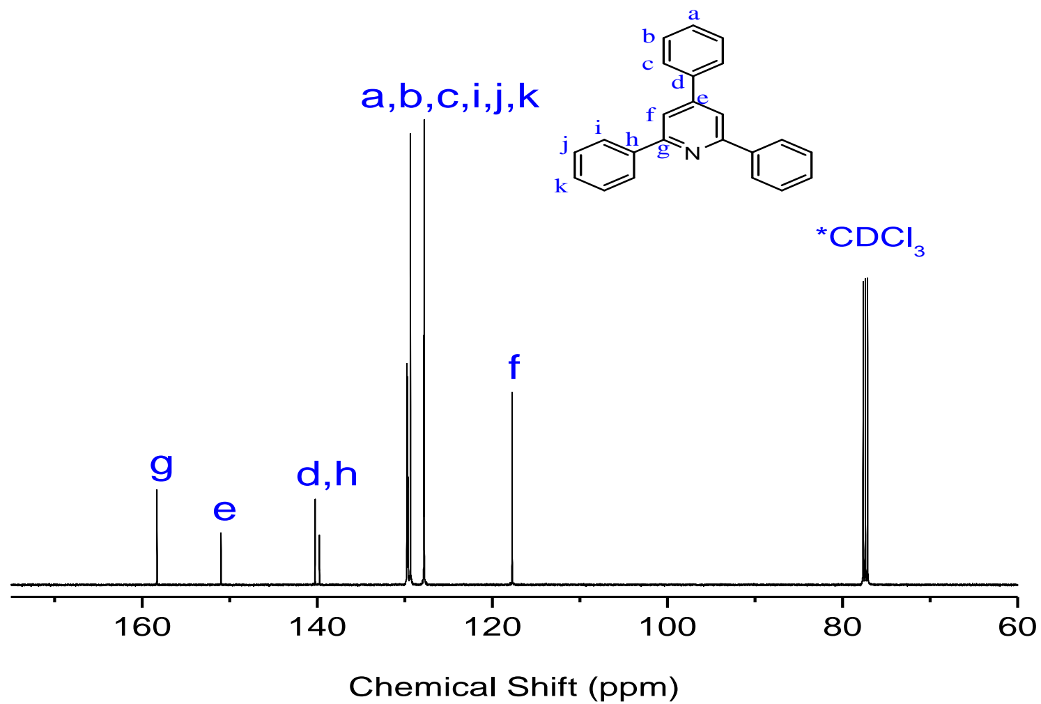
Fig. S2 ^{13}\text{C} NMR of TPP( \text{CDCl}_3 ).
