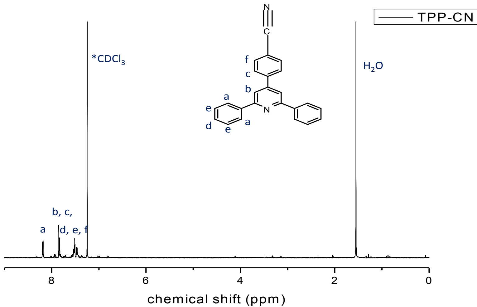
Fig. S3 ^1\text{H} NMR spectrum of TPP-CN( \text{CDCl}_3 ).
