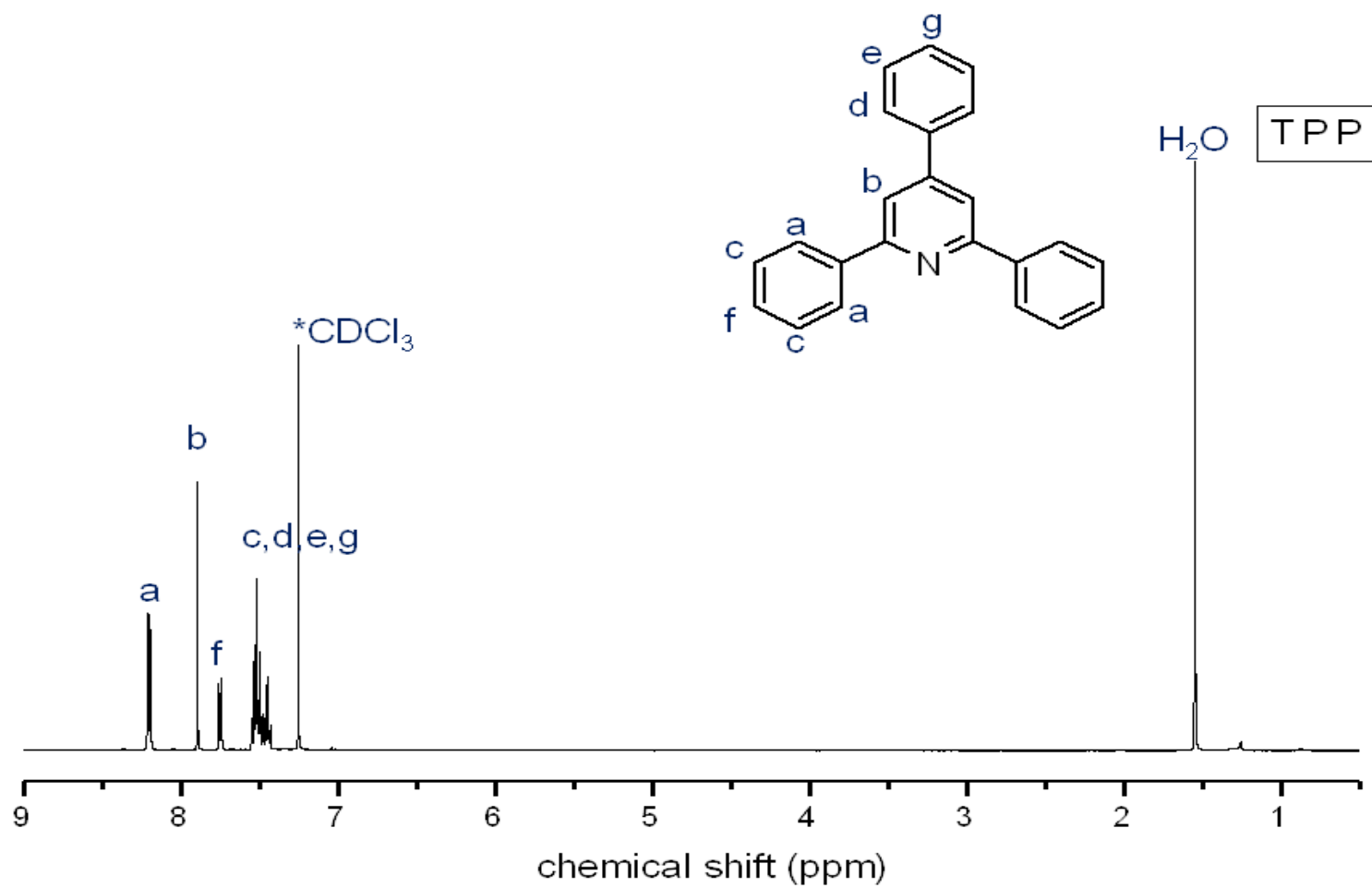
Fig. S1 ^1\text{H} NMR of TPP( \text{CDCl}_3 ).
