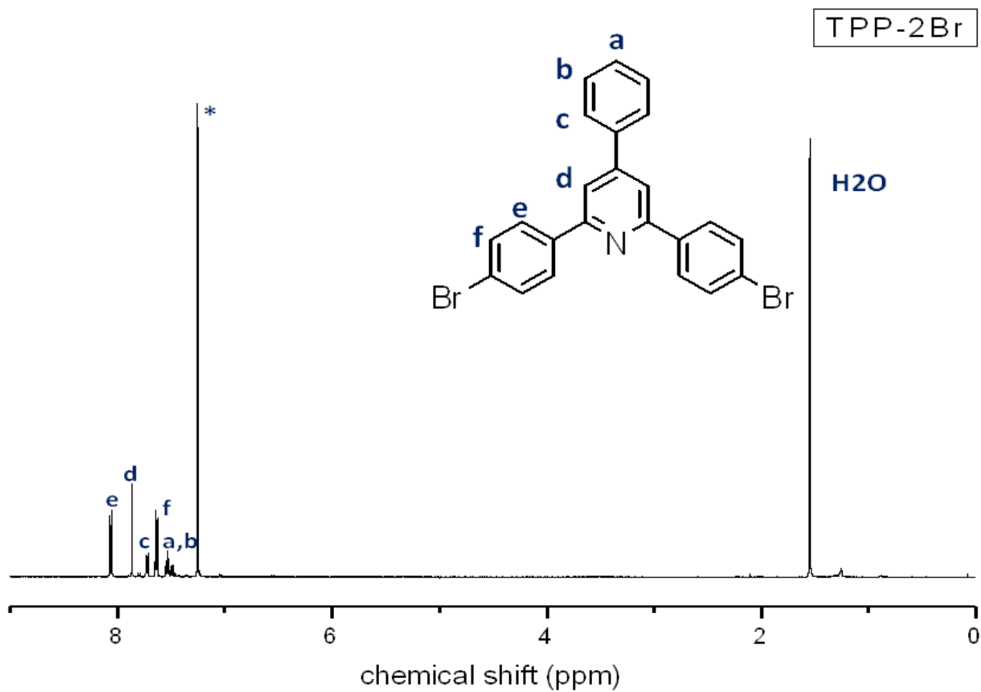
Fig. S5 ^1\text{H-NMR} spectrum of TPP-2Br( \text{CDCl}_3 ).
