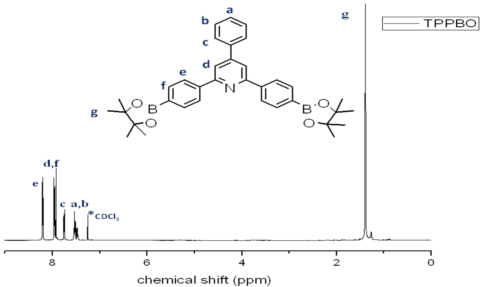
Fig. S6 1 H-NMR spectrum of TPPBO(CDCl 3 ).
