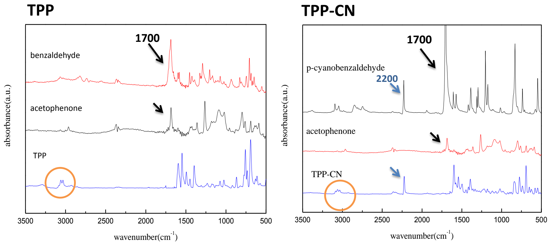
Fig. S11 FT-IR spectra of TPP and TPP-CN.
