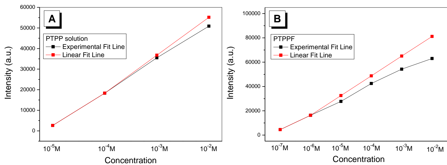
Fig. S13 The intensity-concentration curves spectra of (A) PTPP and (B) PTPPF.
