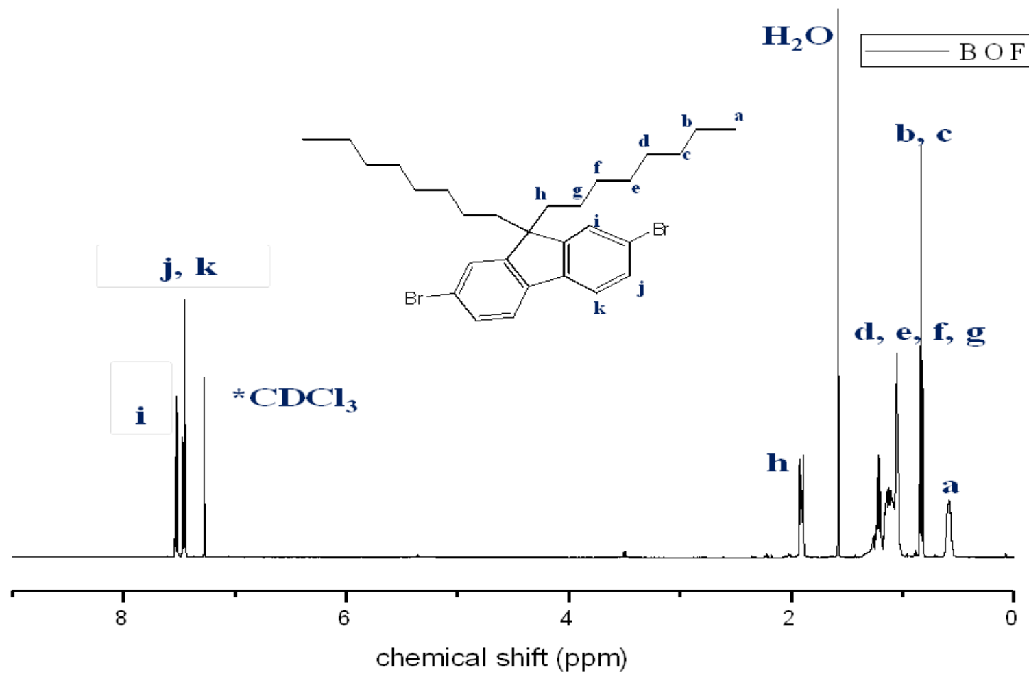
Fig. S7 ^1\text{H-NMR} spectrum of DOF ( \text{CDCl}_3 ).
