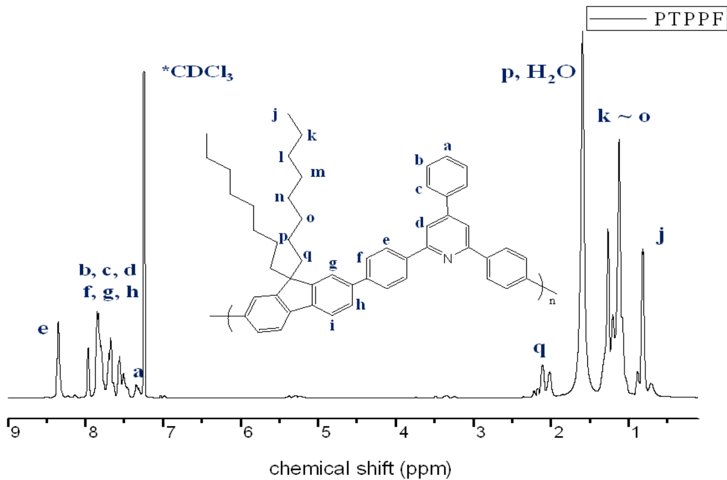
Fig. S9 ^1\text{H-NMR} spectrum of PTPPF( \text{CDCl}_3 ).
