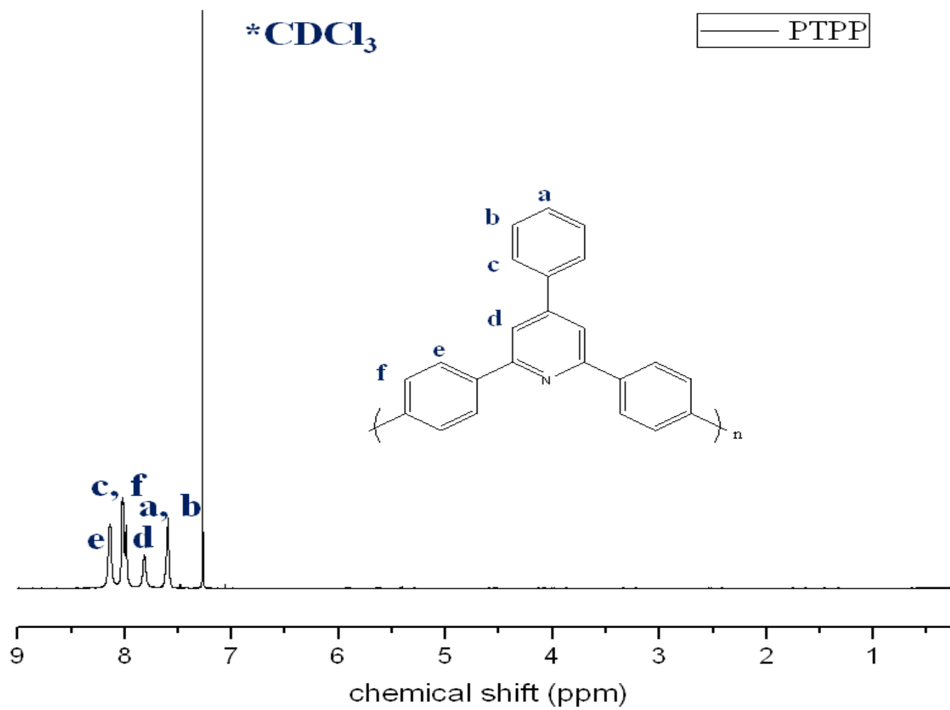
Fig. S8 ^1\text{H-NMR} spectrum of PTPP( \text{CDCl}_3 ).
