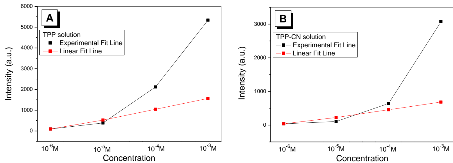
Fig. S12 The intensity-concentration curves spectra of (A) TPP and (B) TPP-CN.
