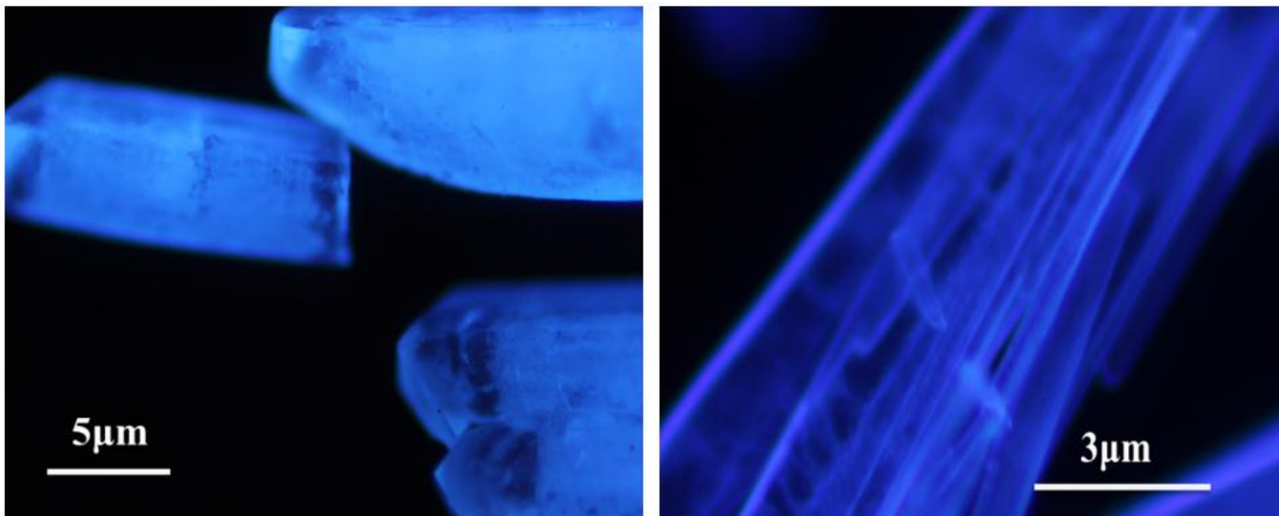
Fig. S10 Fluorescent images of TPP (left) and TPP-CN (right) obtained by slow evaporations from the THF/hexane solutions.
