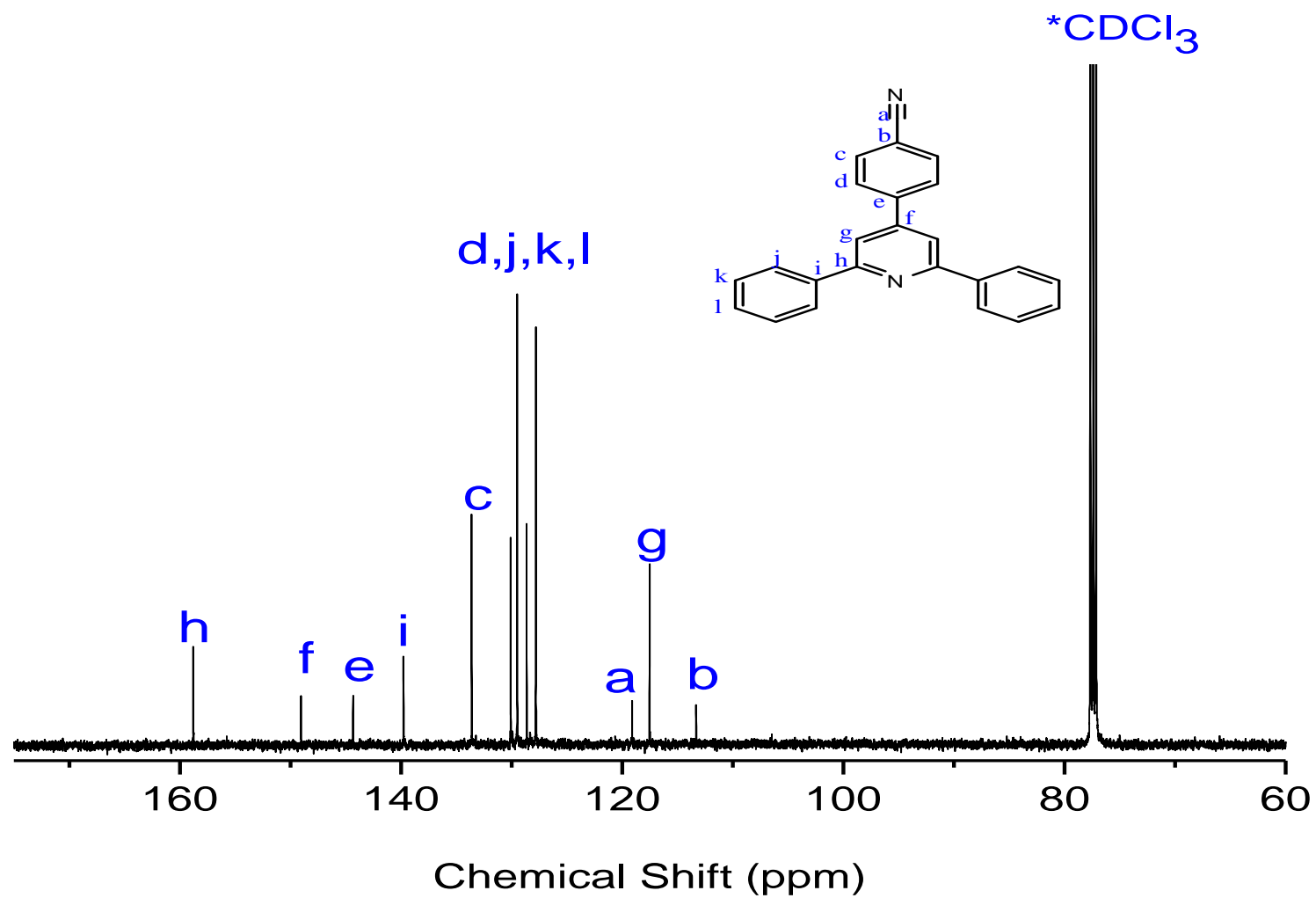
Fig. S4 ^{13}\text{C} NMR of TPP-CN( \text{CDCl}_3 ).
