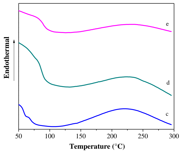
Fig. S1 DSC curves of the cured PNCs with (c) 1.0 wt% BaTiO 3 (500 nm), (d) 5.0 wt% BaTiO 3 (500 nm), and (e) 10.0 wt% BaTiO 3 (500 nm).
