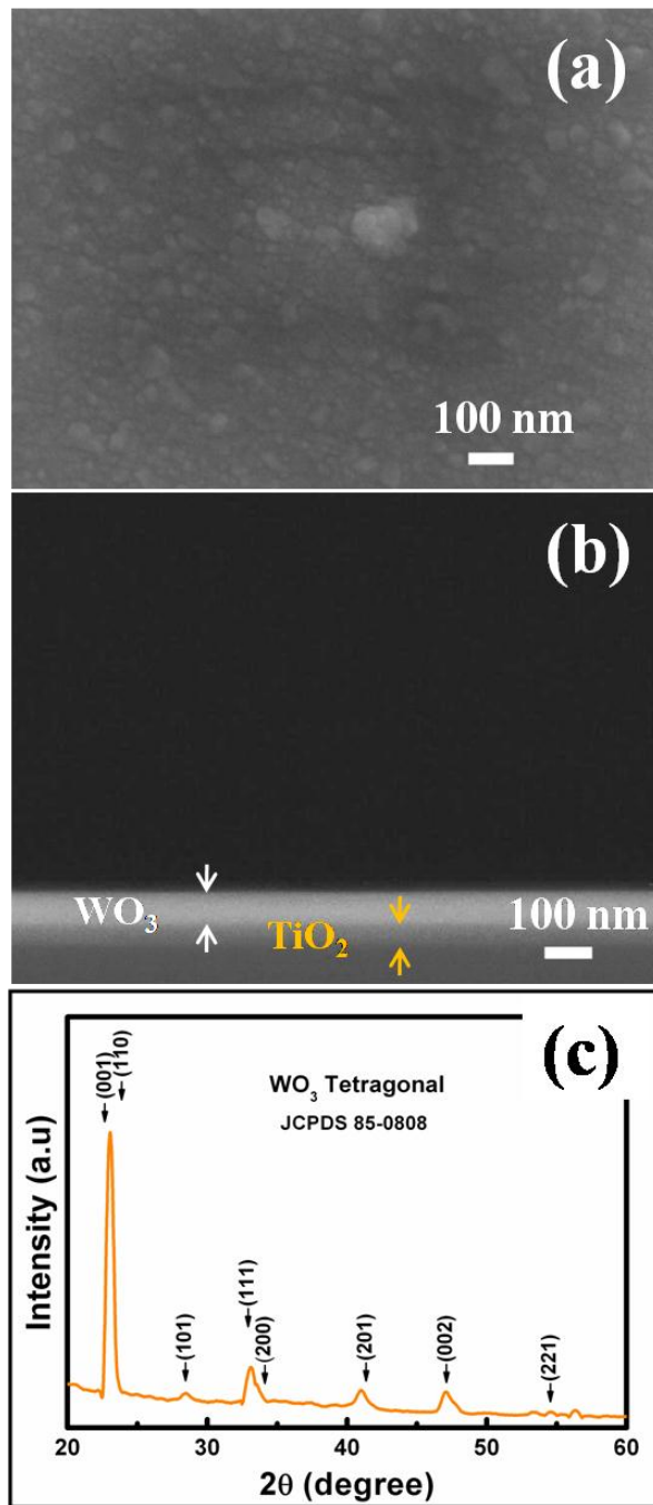
5 Fig. S1. SEM images of \text{WO}_3 – \text{TiO}_2 composite thin film. (a) Top view and (b) cross – section view. (c) XRD pattern of the thin film only showed peaks for tetragonal \text{WO}_3 .
