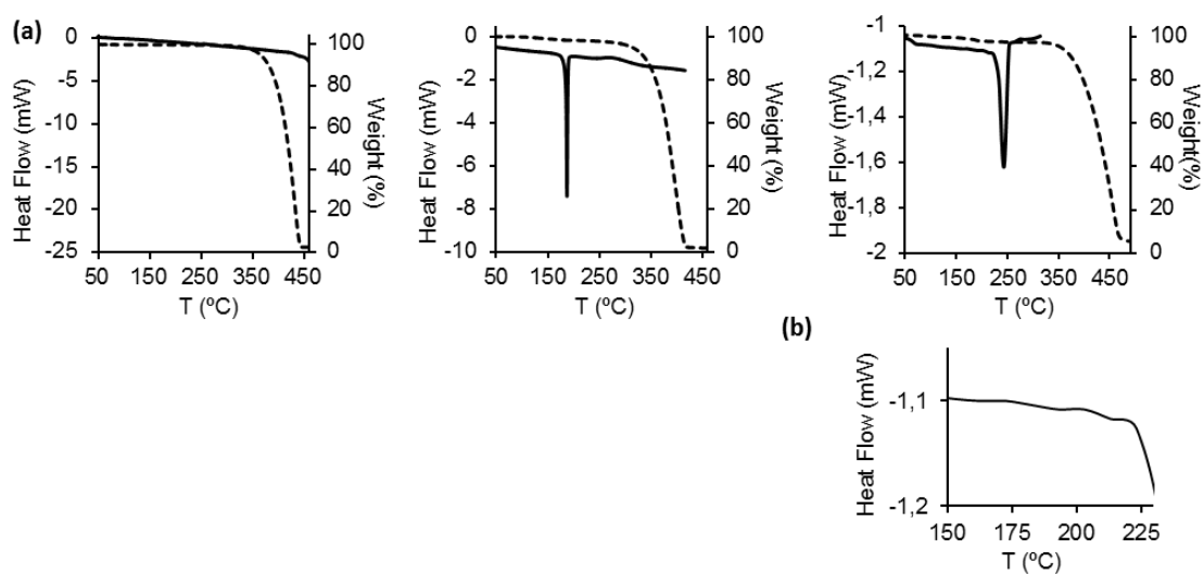
Fig. 1 (a) Thermogravimetric Analysis (dashed line) and Differential Scanning Calorimetry (continuous line) of compounds 1 (left), 2 (centre) and 3 (right). (b) Expanded thermogram.
