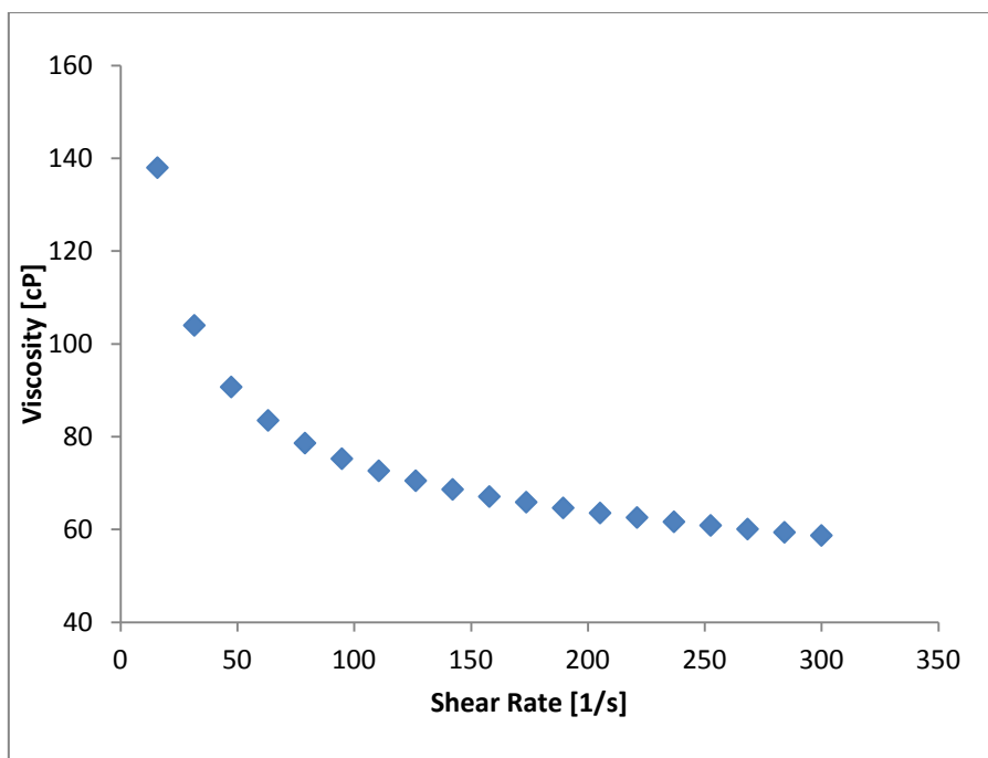
Viscosity vs. shear rate dependence for an ink containing 20% Ag nanoparticles
