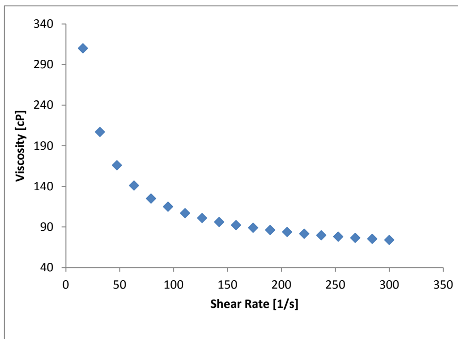
Viscosity vs. shear rate dependence for an ink containing 30% Ag nanoparticles
