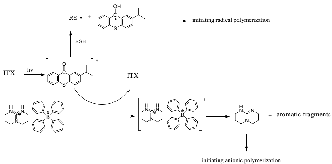
Scheme 1. Photolysis of ITX/ TBD•HBPh4.
