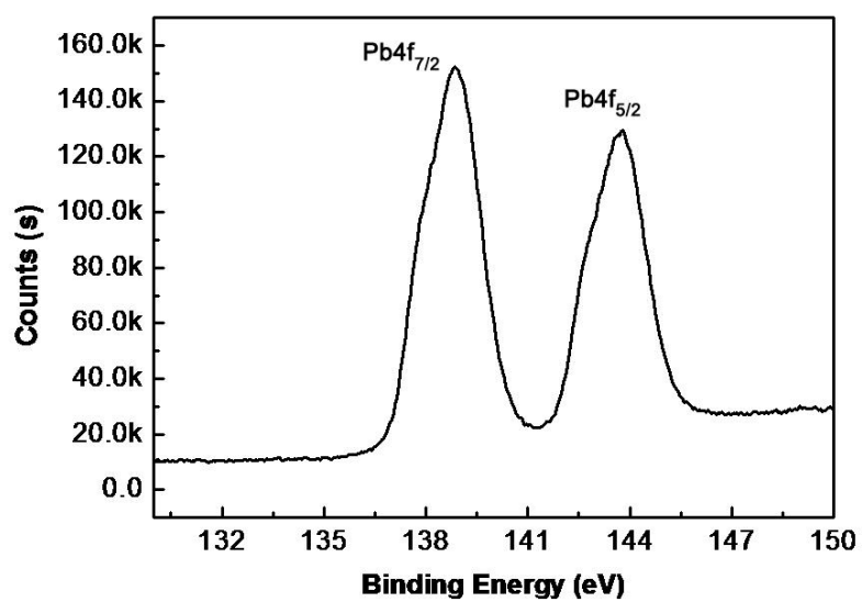
Fig. S1 XPS spectrum of the Pb4f region for the CdTe micropattern reacted with a Pb 2+ solution.
