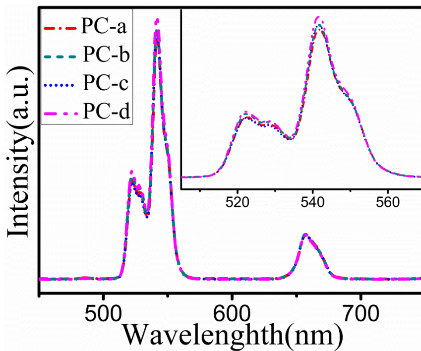
Fig.2 the UC emission spectra of \text{NaYF}_4:\text{Yb}^{3+}, \text{Er}^{3+} on the surface of PC-II with the various thicknesses
