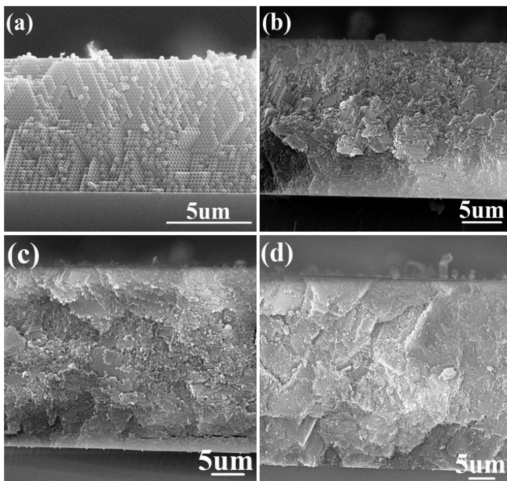
Fig.1 the cross-section SEM images of PC-II photonic crystal with various thicknesses
