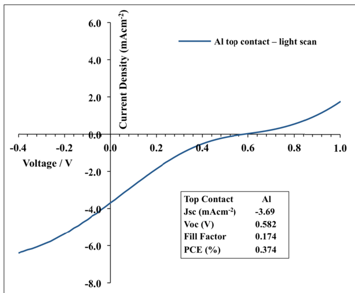
Figure S2 - Current density-voltage (J-V) plot for a conventional Al top contact organic solar cell ITO/PEDOT:PSS/P3HT/PCBM/Al with measured device parameters.
