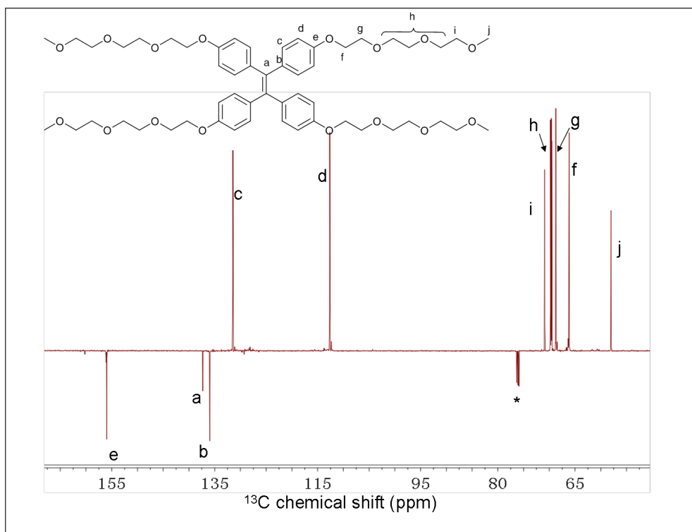
Figure S1. ^{13}\text{C} NMR spectra of \text{M}(\text{EO})_3\text{-TPE} in \text{CDCl}_3 .
