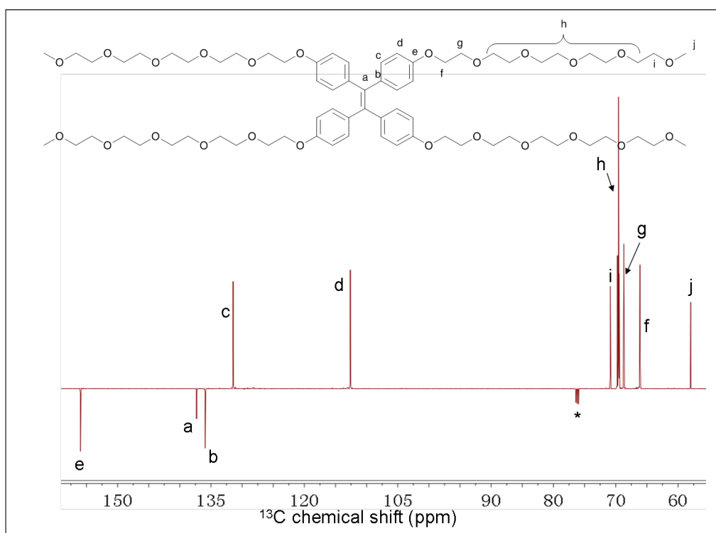
Figure S3. ^{13}\text{C} NMR spectra of \text{M}(\text{EO})_5\text{-TPE} in \text{CDCl}_3 .
