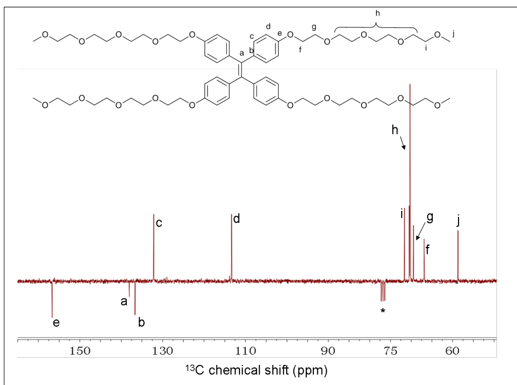
Figure S2. ^{13}\text{C} NMR spectra of \text{M}(\text{EO})_4\text{-TPE} in \text{CDCl}_3 .
