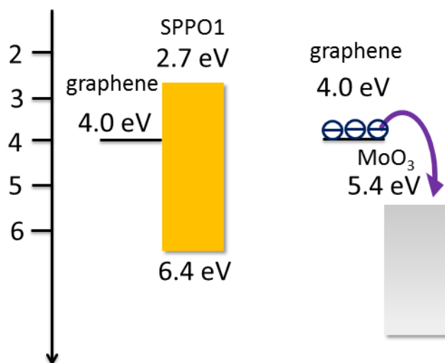
Figure S2. Energy band diagram of graphene and SPPO1. The band structure of graphene and MoO 3 is also illustrated for comparison.
