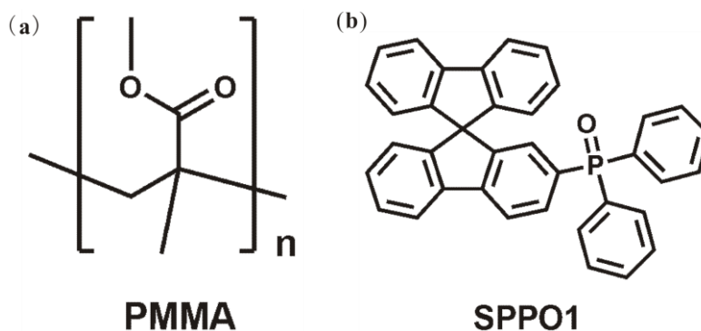
Figure S1. The molecular structures of (a) PMMA and (b) SPPO1.
