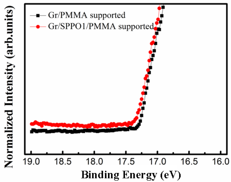
Figure S3. UPS spectra of G-P and G-PS.
