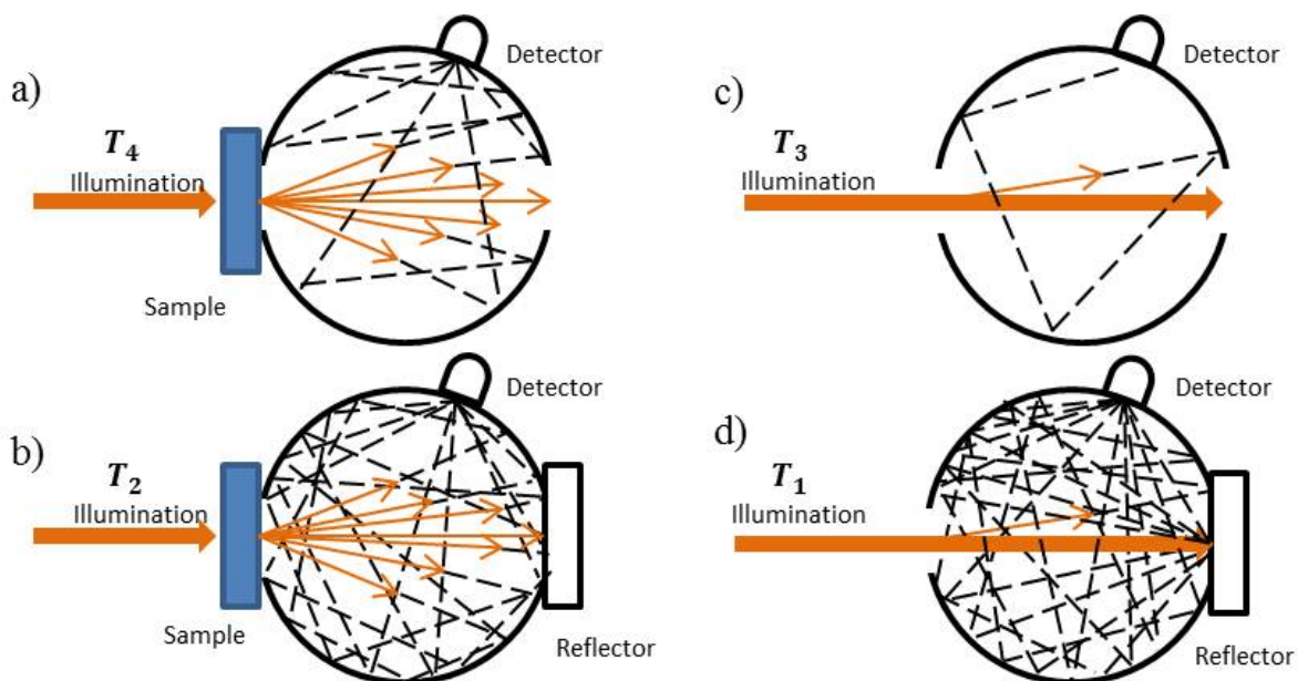
S3) The experimental haze measurement setup with the UV-Vis spectrometer, (a) total forward scattered illumination, (b) total transmitted illumination, (c) and (d) are the corrections for the experimental setup.
