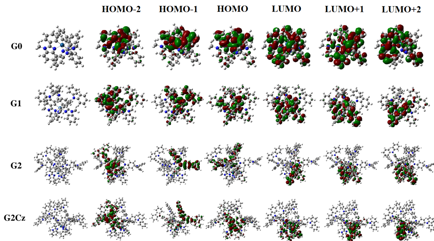
Fig. S1 Selected frontier orbitals for the complexes.
