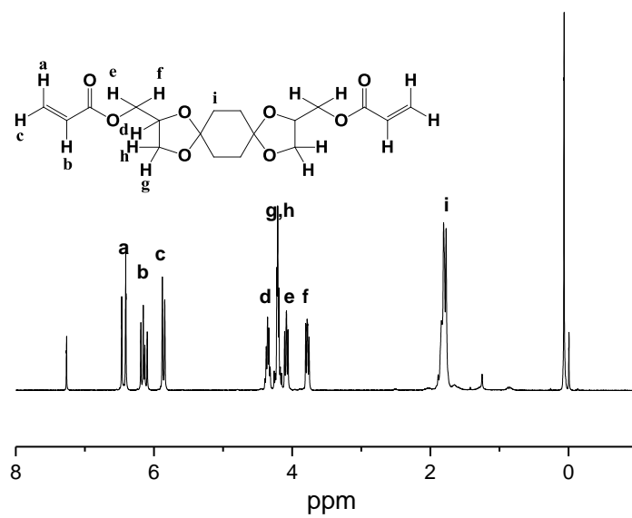
1 H NMR spectra of DAMTT
