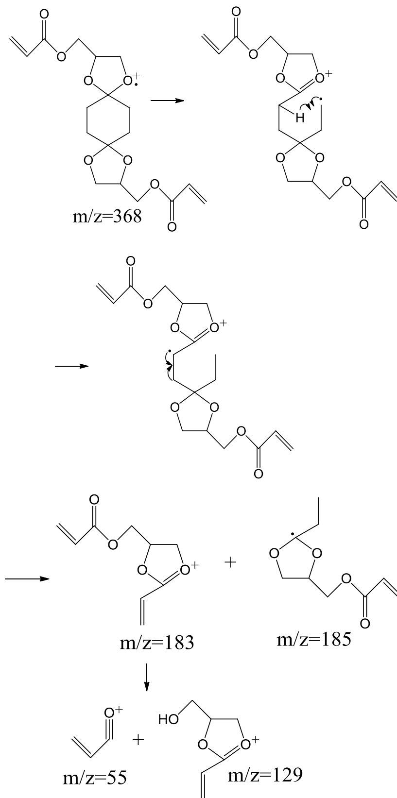
GC-MS fragmentation mechanism of DAMTT
