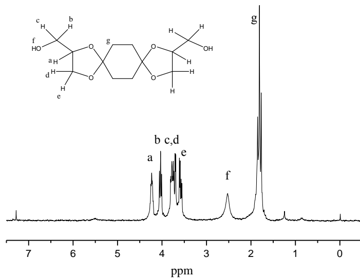
1 H NMR spectra of DHMTT
