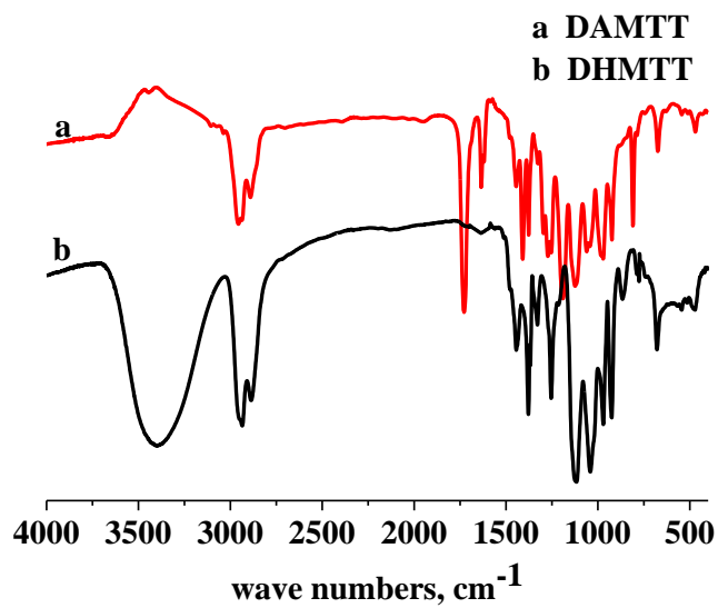
FTIR spectrum of DHMTT and DAMTT
