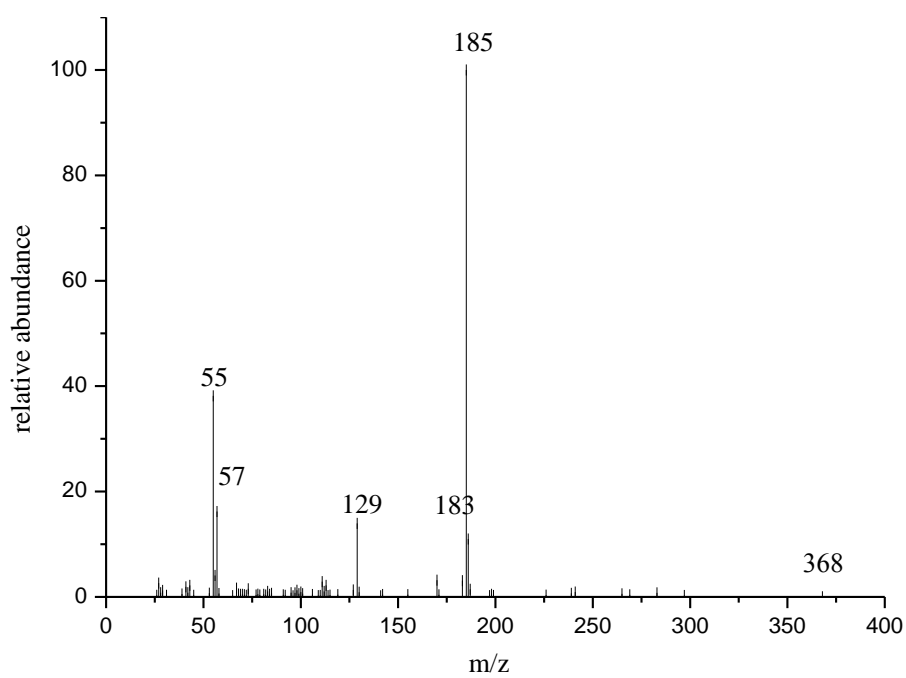
GC-MS of DAMTT
